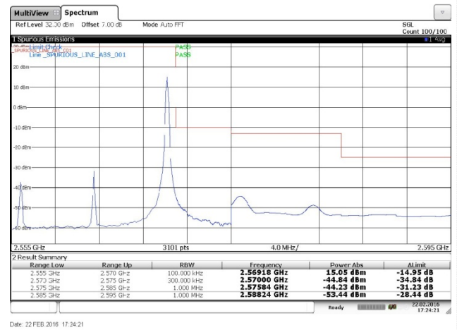
Channel High-1RB#
