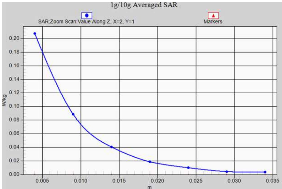
Wi-Fi 802.11b RIGHT/CHEEK-Mid_ axis scan
