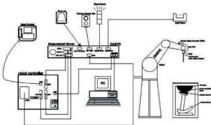
Figure 1 System Diagram
