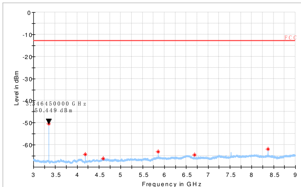
Fig.26 GSM850 on Channel 190 3GHz~9GHz
