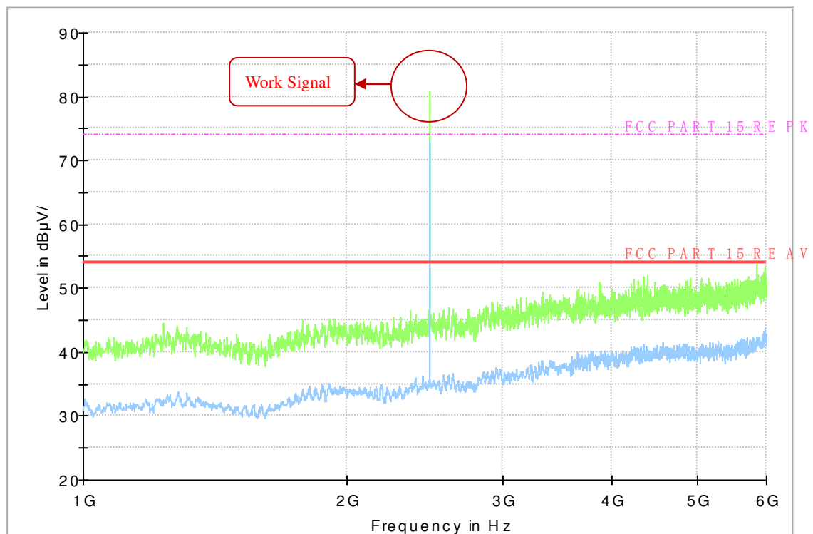
Fig.69 Radiated Emission of channel 78 in 1GHz-6GHz
