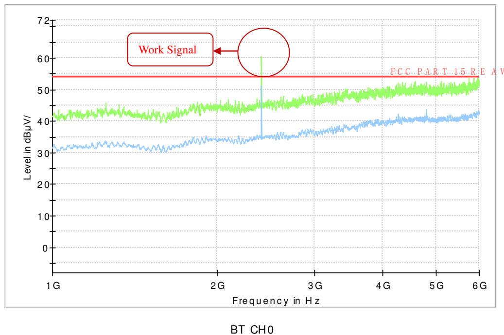
Fig.19 Radiated Emission of channel 0 in 1GHz-6GHz
