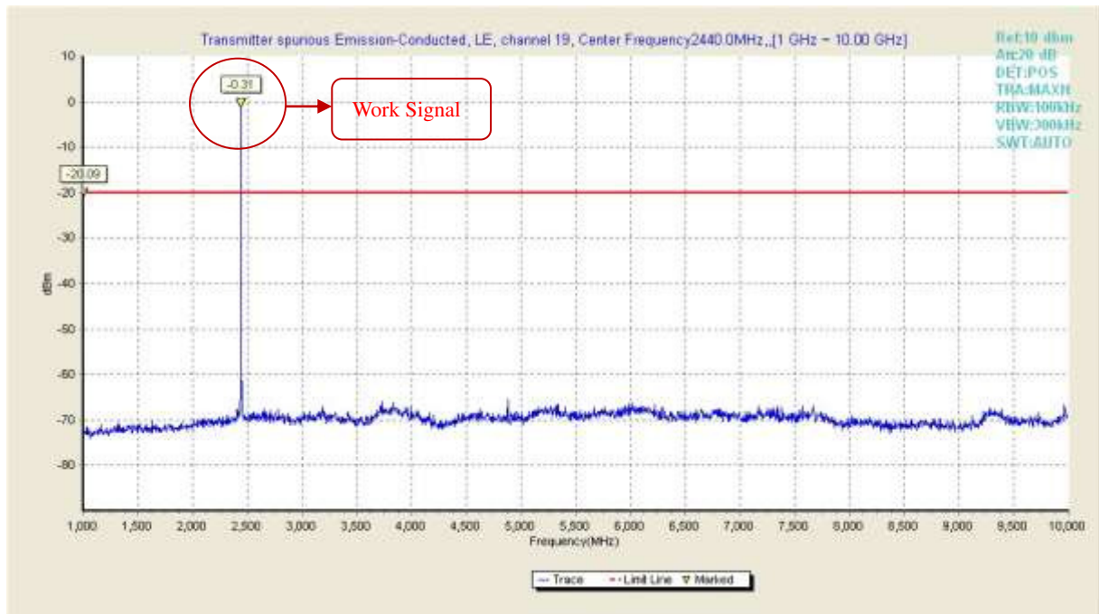
Fig.13 Transmitter spurious emission-Conducted of BLE in channel 19,( 1GHz ~10GHz)
