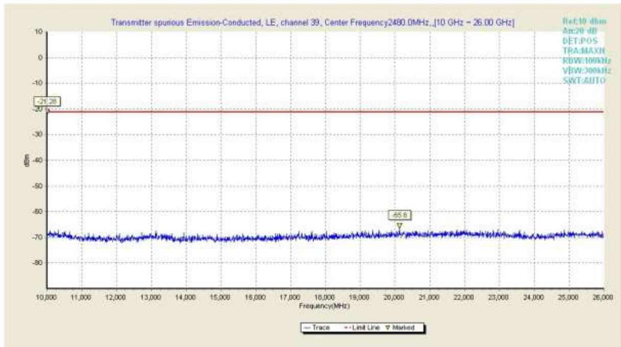
Fig.17 Transmitter spurious emission-Conducted of BLE in channel 39,( 10GHz ~26GHz)
