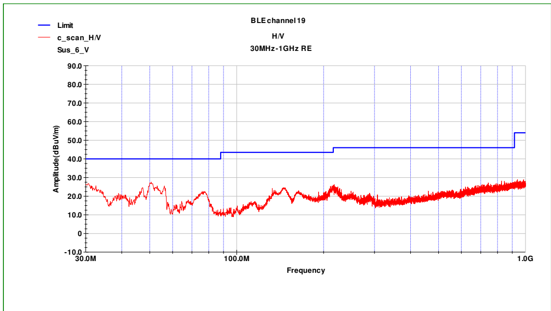
Fig.20 Radiated Emission of channel 19 in 30MHz-1GHz
