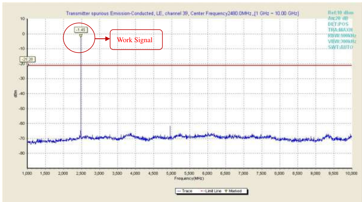
Fig.16 Transmitter spurious emission-Conducted of BLE in channel 39,( 1GHz ~10GHz)
