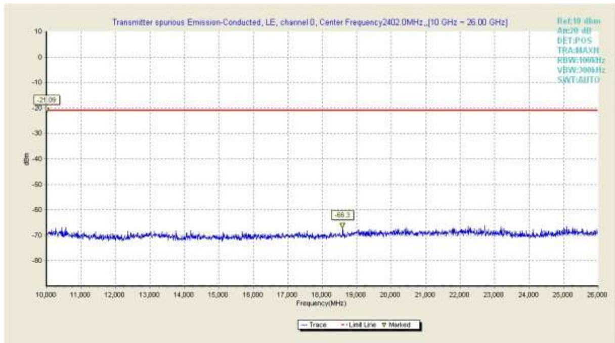
Fig.11 Transmitter spurious emission-Conducted of BLE in channel 0,( 10GHz ~26GHz)
