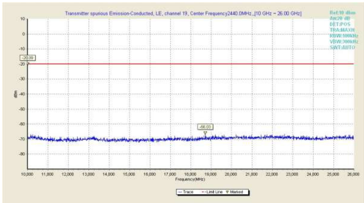
Fig.14 Transmitter spurious emission-Conducted of BLE in channel 19,( 10GHz ~26GHz)
