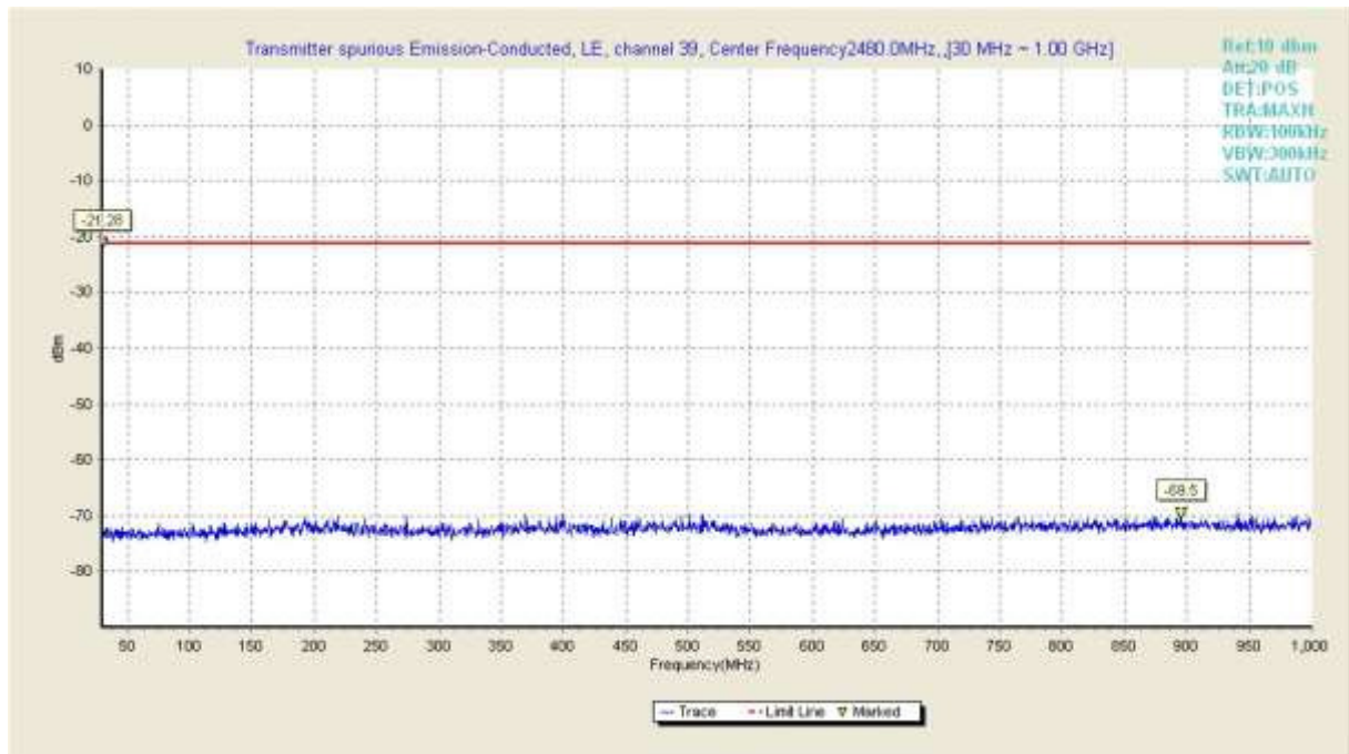
Fig.15 Transmitter spurious emission-Conducted of BLE in channel 39,( 30MHz ~1GHz)
