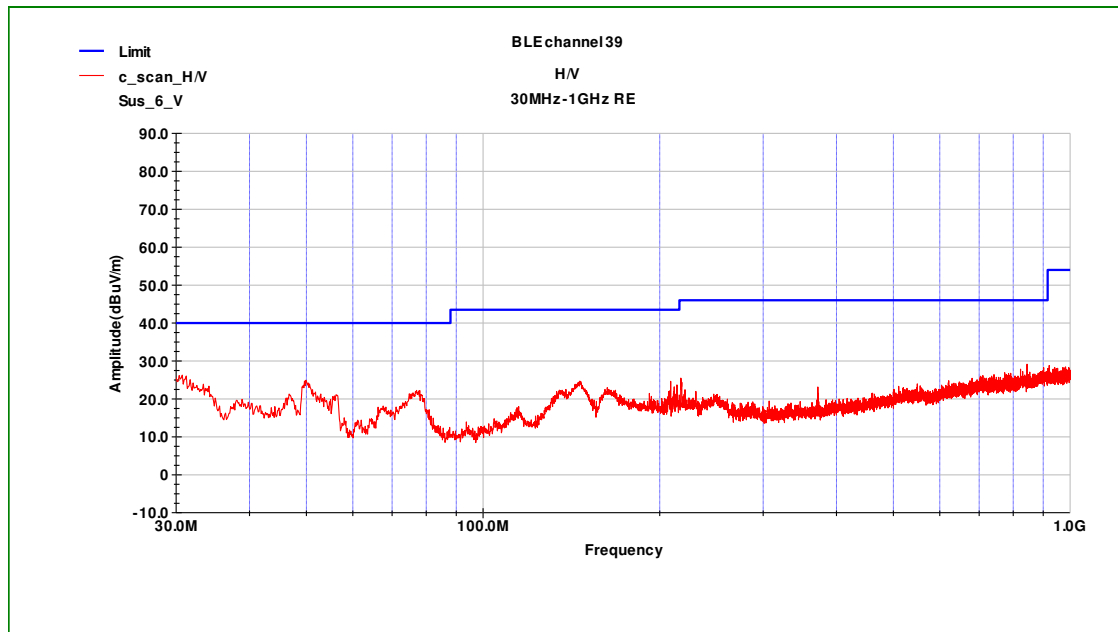
Fig.22 Radiated Emission of channel 39 in 30MHz-1GHz
