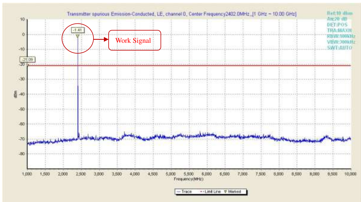
Fig. 10 Transmitter spurious emission-Conducted of BLE in channel 0,( 1GHz ~10GHz)
