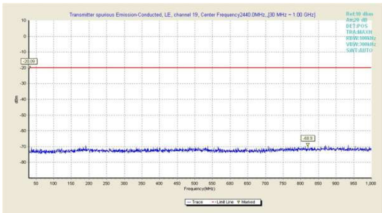
Fig.12 Transmitter spurious emission-Conducted of BLE in channel 19,(30MHz ~1GHz)
