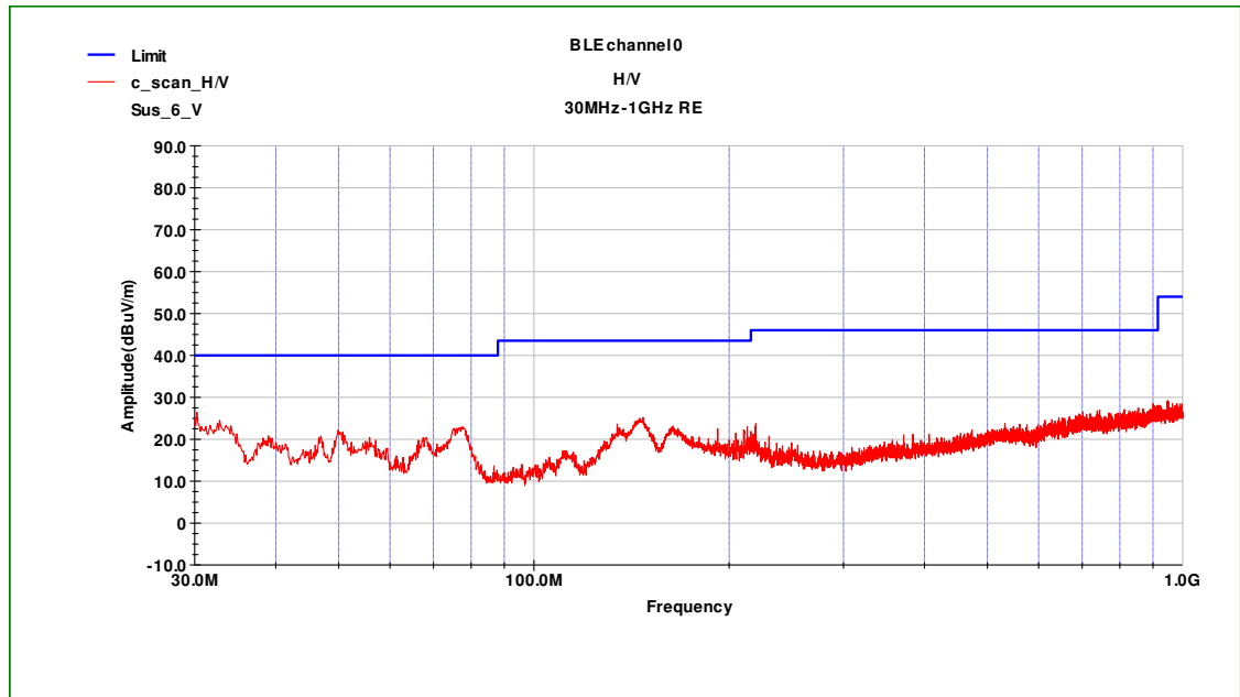
Fig.18 Radiated Emission of channel 0 in 30MHz-1GHz
