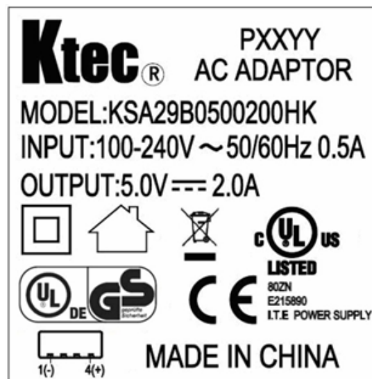
Adapter 2 label view
