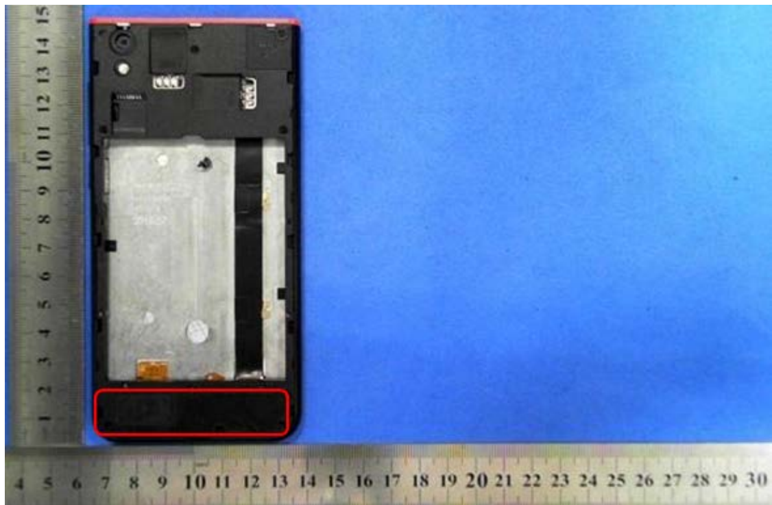
GSM/WCDMA Antenna View
