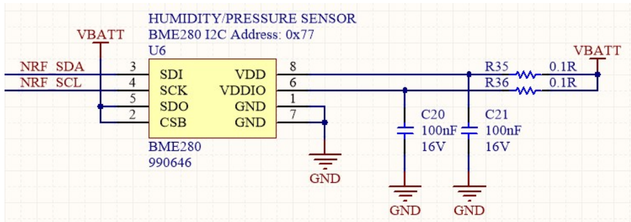
Figure 3-1: Humidity Schematic
