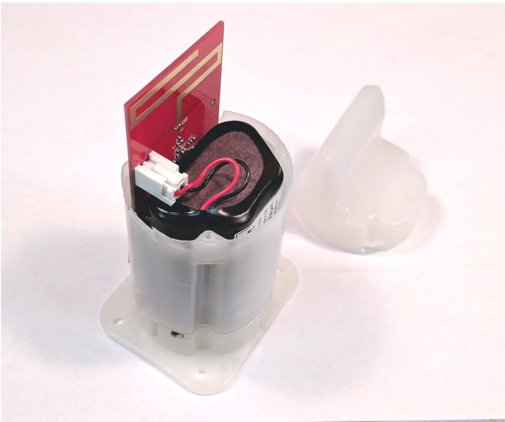
Figure 4: PECO enclosure, Overview, Cap removed:
