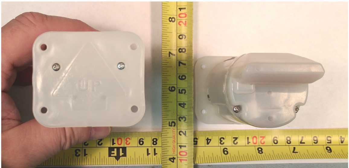
Figure 2: PECO enclosure, Bottom and Top:
