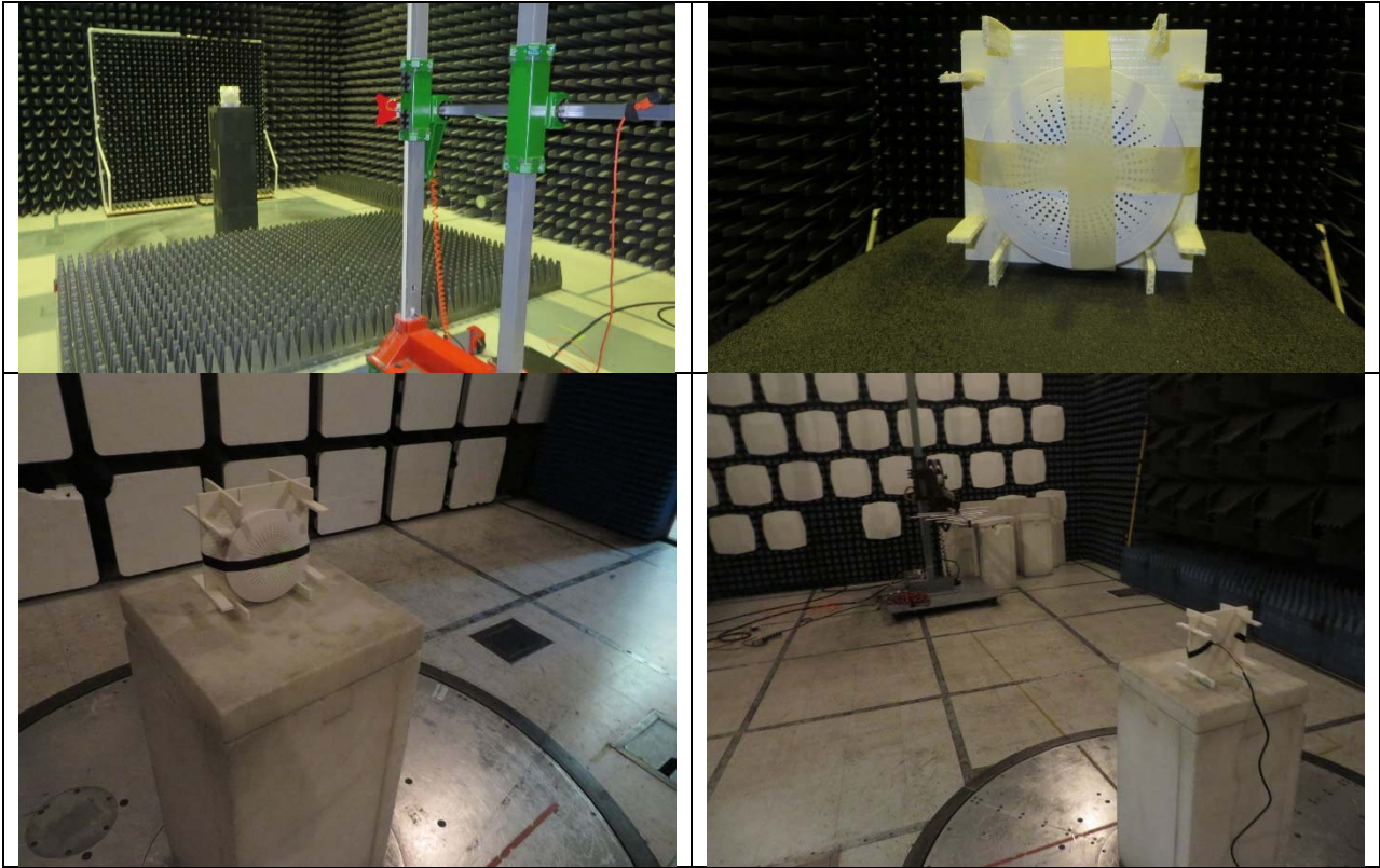
Radiated emissions
