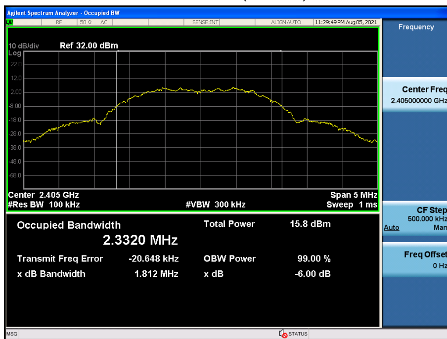
6dB Occupied Bandwidth Mode 1 / CH11 (2405MHz)
