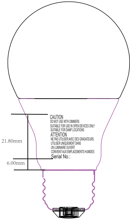
RIGHT SIDE
