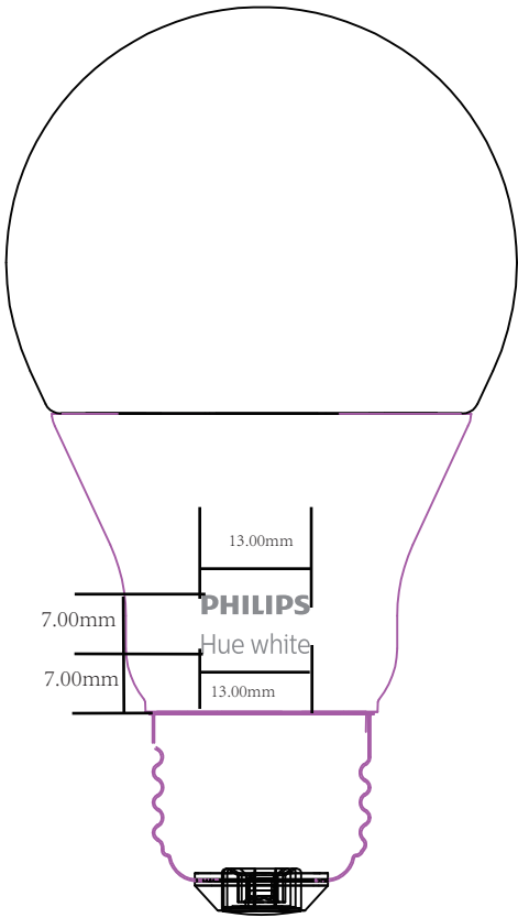
FRONT SIDE
