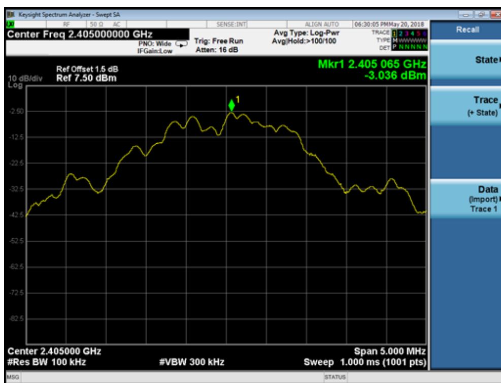
Mode 1 CH11(2405MHz)
