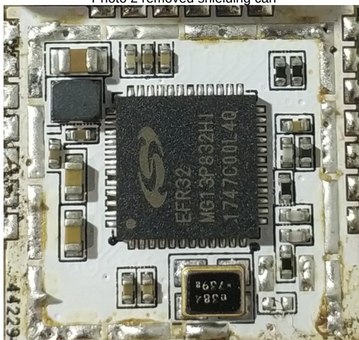
Photo 2 removed shielding can
