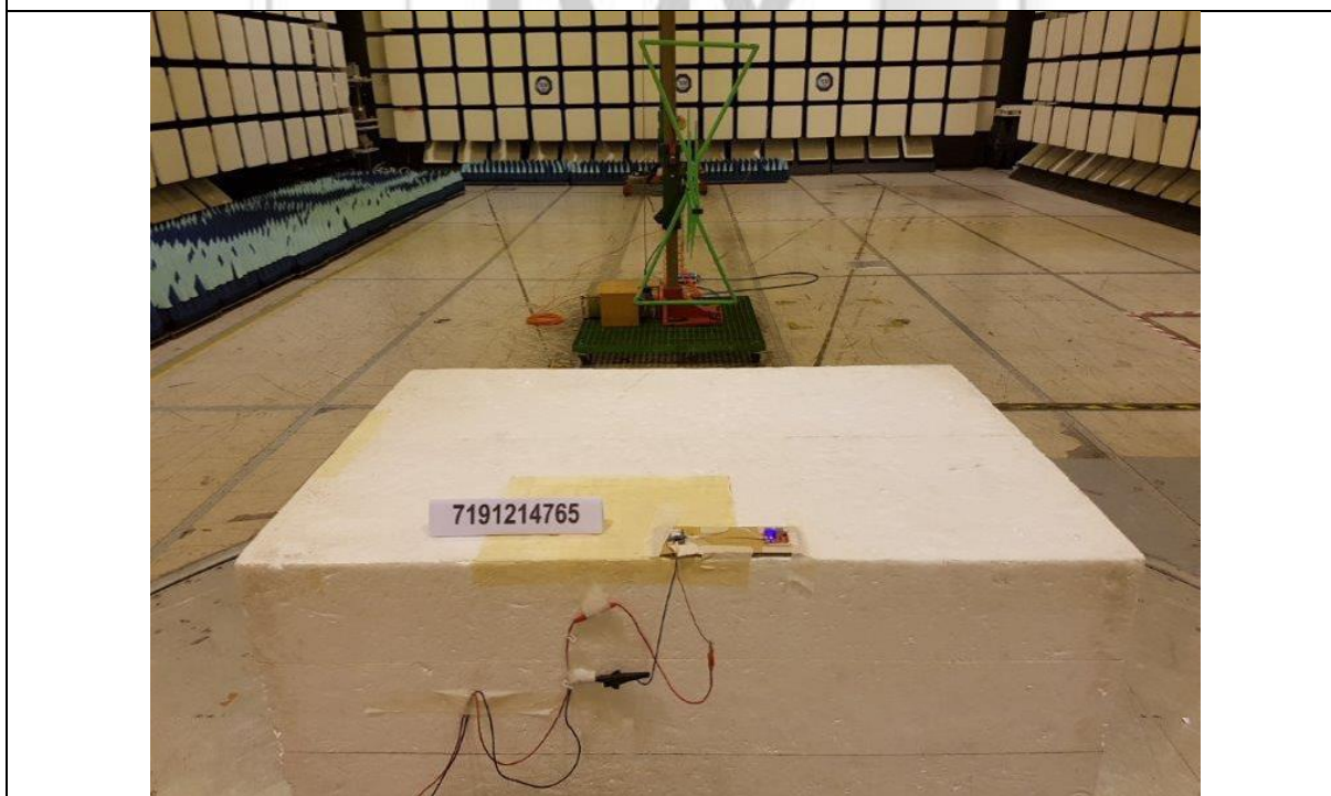
Radiated Emissions (Spurious Emissions Inclusive Restricted Bands Requirement) Test Setup (Rear View)
