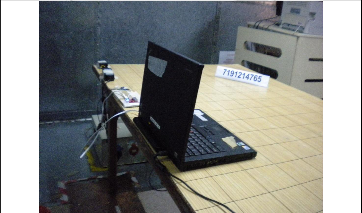
Conducted Emissions Test Setup (Rear View)
