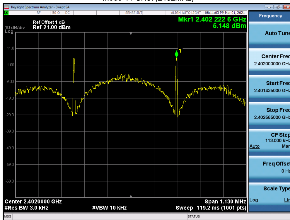
Mode 4 / CH37(2402MHz)
