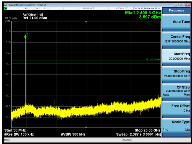
Mode 1 / CH11(2405MHz)
