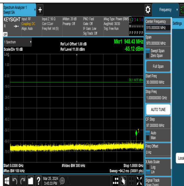
ZIGB-Ant1-2405-30~1000-PASS
