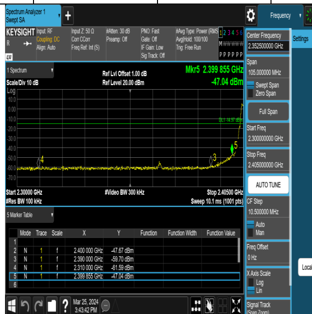
ZIGB-Ant1-2405-PASS
