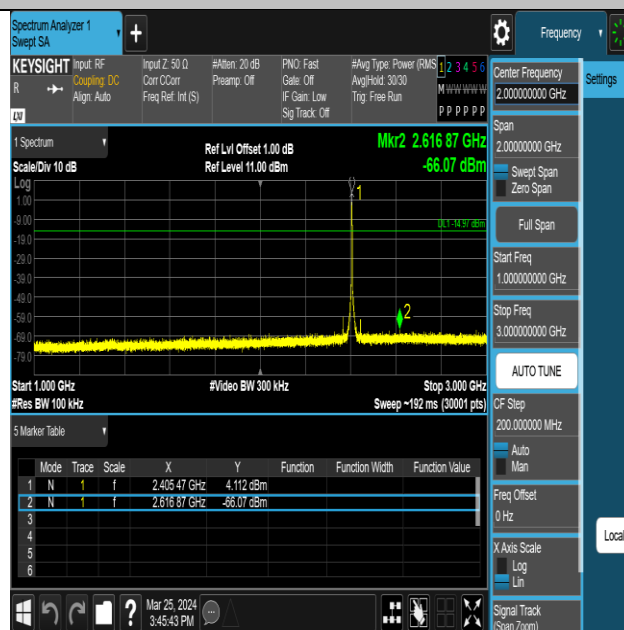
ZIGB-Ant1-2405-1000~3000-PASS
