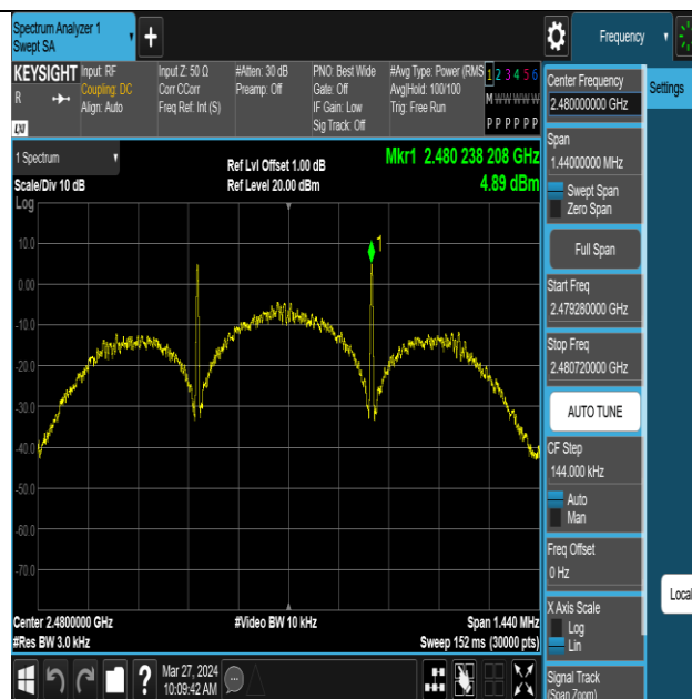
BLE_125K-Ant1-2480-PASS
