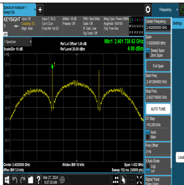
BLE_125K-Ant1-2402-PASS
