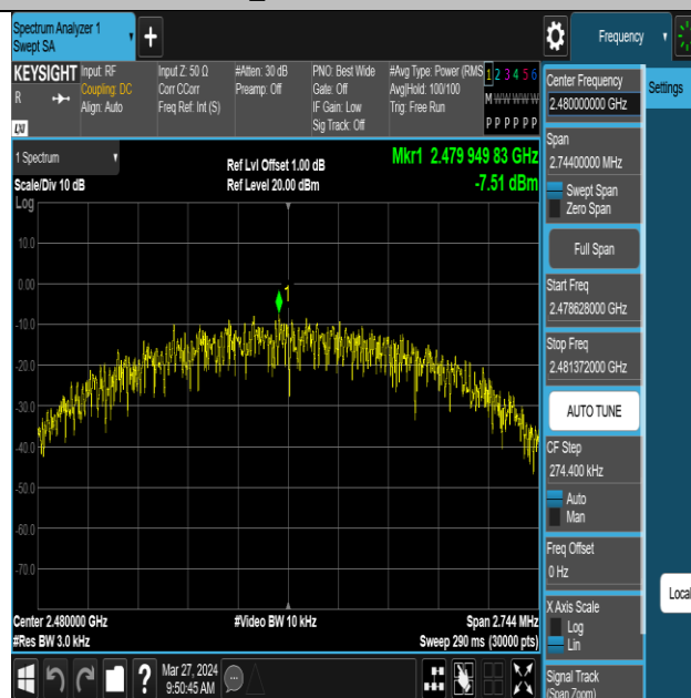
BLE_2M-Ant1-2480-PASS
