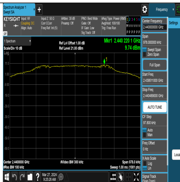
BLE_1M-Ant1-2440-PASS
