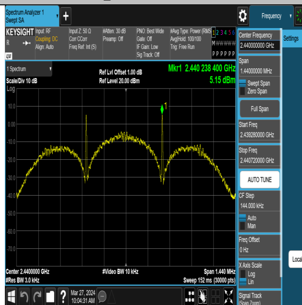
BLE_125K-Ant1-2440-PASS
