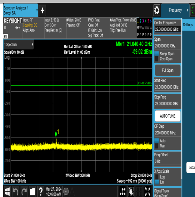
ZIGB-Ant1-2405-21000~23000-PASS
