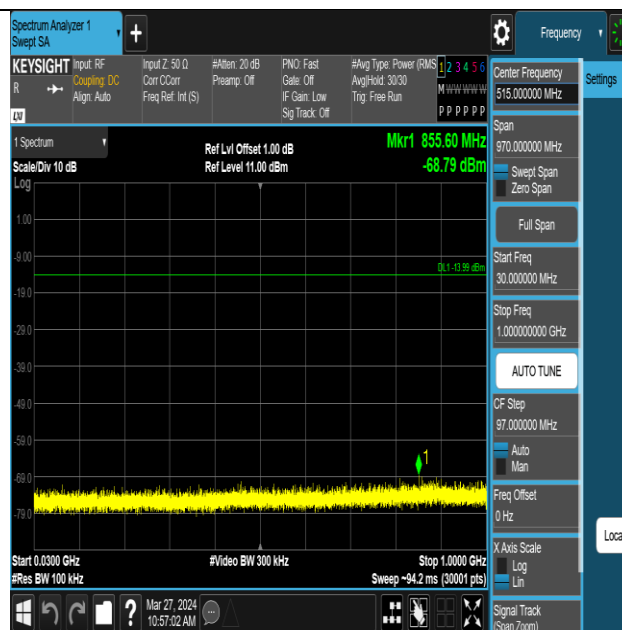
ZIGB-Ant1-2480-30~1000-PASS
