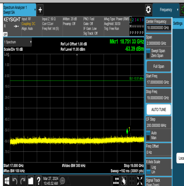
ZIGB-Ant1-2405-17000~19000-PASS
