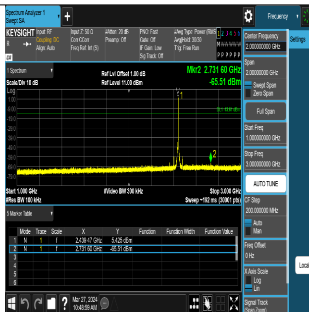
ZIGB-Ant1-2440-1000~3000-PASS
