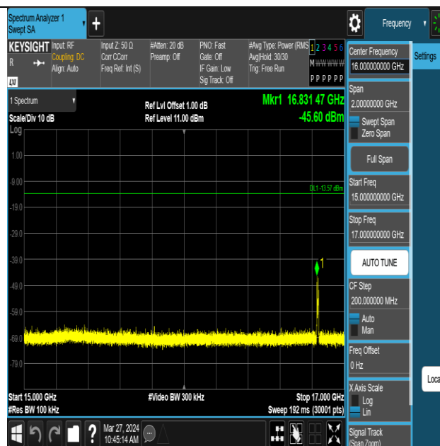
ZIGB-Ant1-2405-15000~17000-PASS
