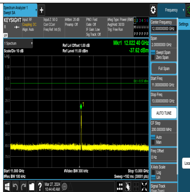
ZIGB-Ant1-2405-11000~13000-PASS
