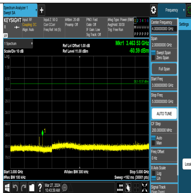
ZIGB-Ant1-2405-3000~5000-PASS
