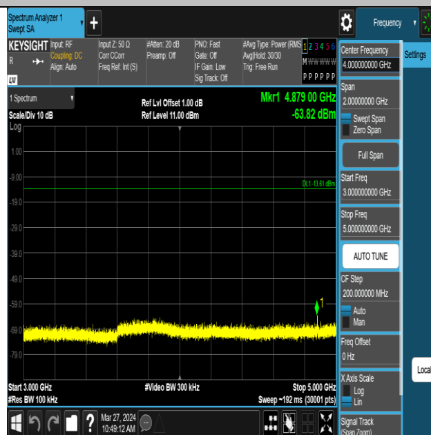
ZIGB-Ant1-2440-3000~5000-PASS
