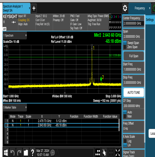
ZIGB-Ant1-2480-1000~3000-PASS
