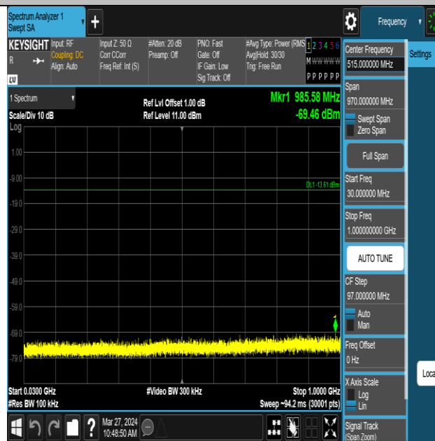
ZIGB-Ant1-2440-30~1000-PASS
