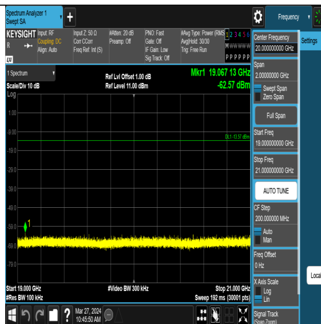
ZIGB-Ant1-2405-19000~21000-PASS
