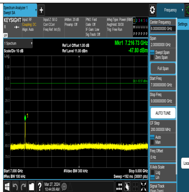
ZIGB-Ant1-2405-7000~9000-PASS
