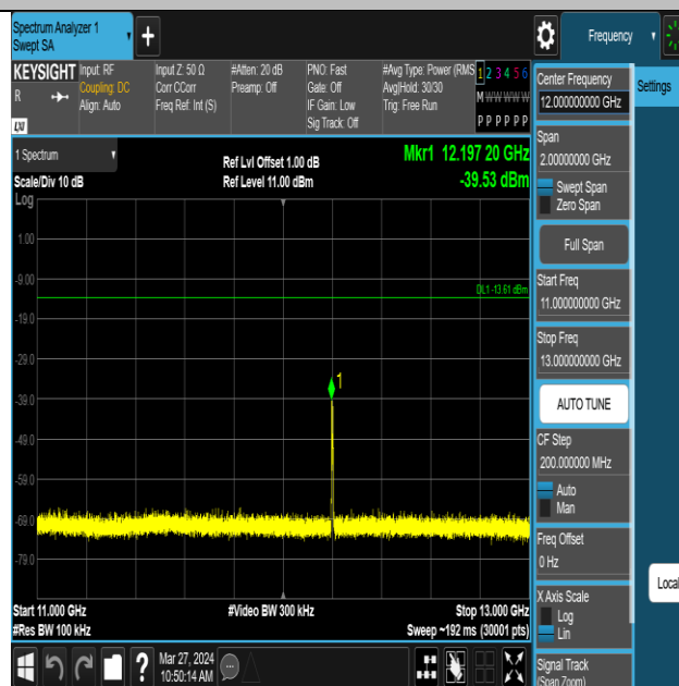
ZIGB-Ant1-2440-11000~13000-PASS
