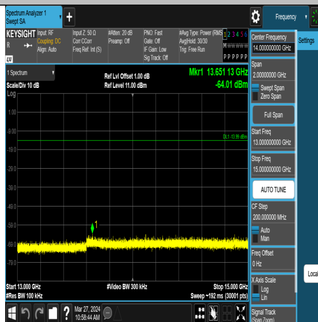
ZIGB-Ant1-2480-13000~15000-PASS
