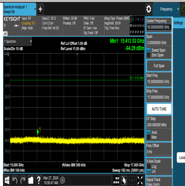
ZIGB-Ant1-2440-15000~17000-PASS
