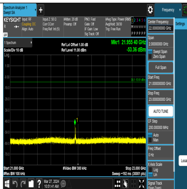
ZIGB-Ant1-2440-21000~23000-PASS
