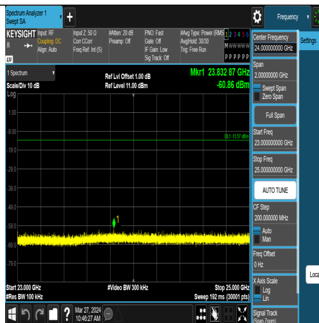
ZIGB-Ant1-2405-23000~25000-PASS
