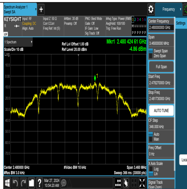
ZIGB-Ant1-2480-PASS
