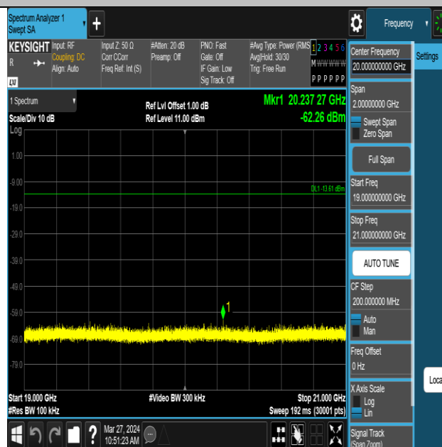
ZIGB-Ant1-2440-19000~21000-PASS
