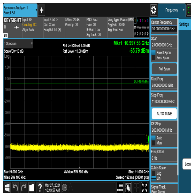
ZIGB-Ant1-2440-9000~11000-PASS
