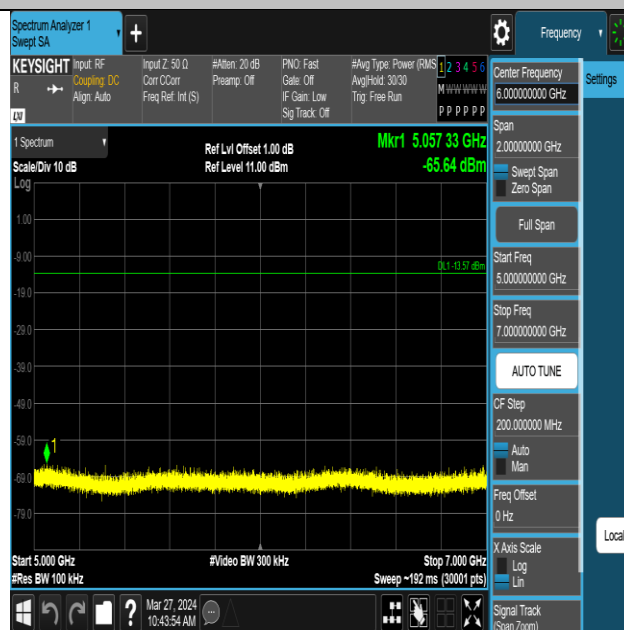
ZIGB-Ant1-2405-5000~7000-PASS
