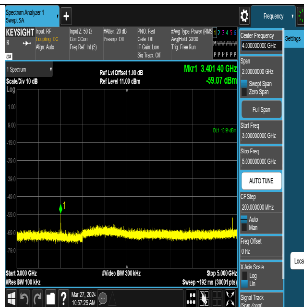
ZIGB-Ant1-2480-3000~5000-PASS
