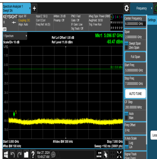
ZIGB-Ant1-2440-5000~7000-PASS
