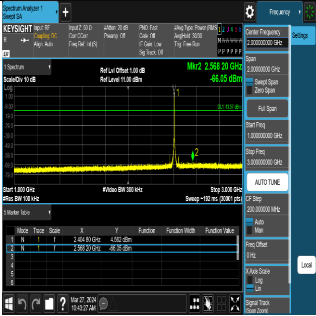
ZIGB-Ant1-2405-1000~3000-PASS
