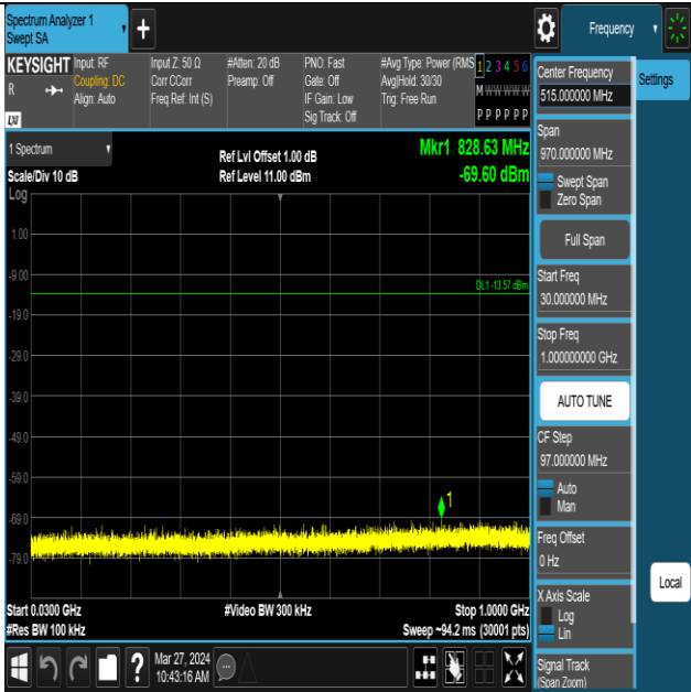
ZIGB-Ant1-2405-30~1000-PASS
