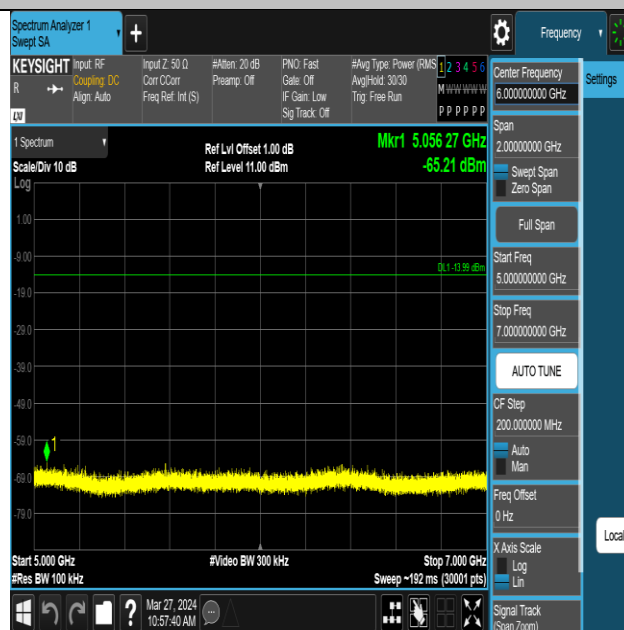
ZIGB-Ant1-2480-5000~7000-PASS
