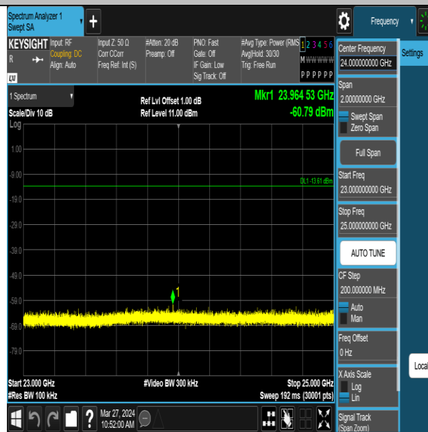
ZIGB-Ant1-2440-23000~25000-PASS
