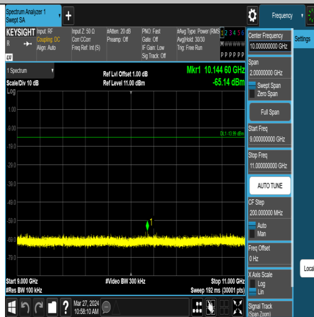
ZIGB-Ant1-2480-9000~11000-PASS
