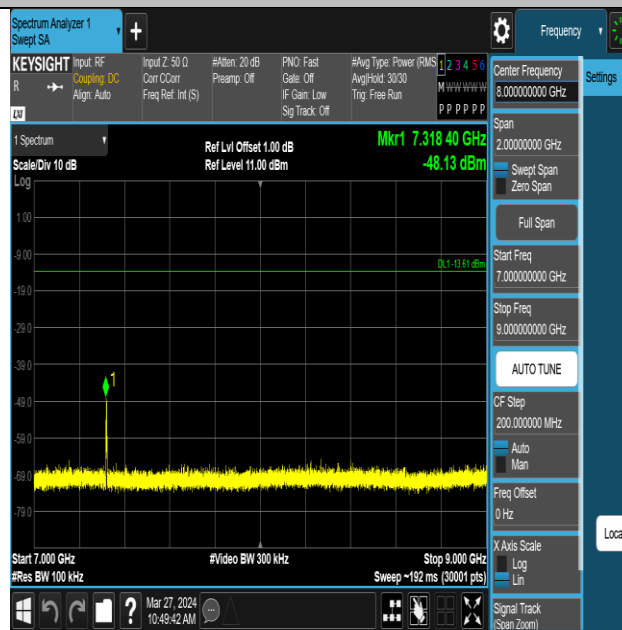
ZIGB-Ant1-2440-7000~9000-PASS
