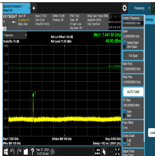
ZIGB-Ant1-2480-7000~9000-PASS
