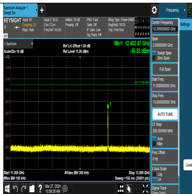
ZIGB-Ant1-2480-11000~13000-PASS
