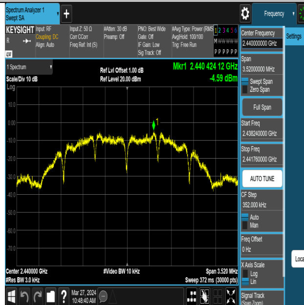
ZIGB-Ant1-2440-PASS
