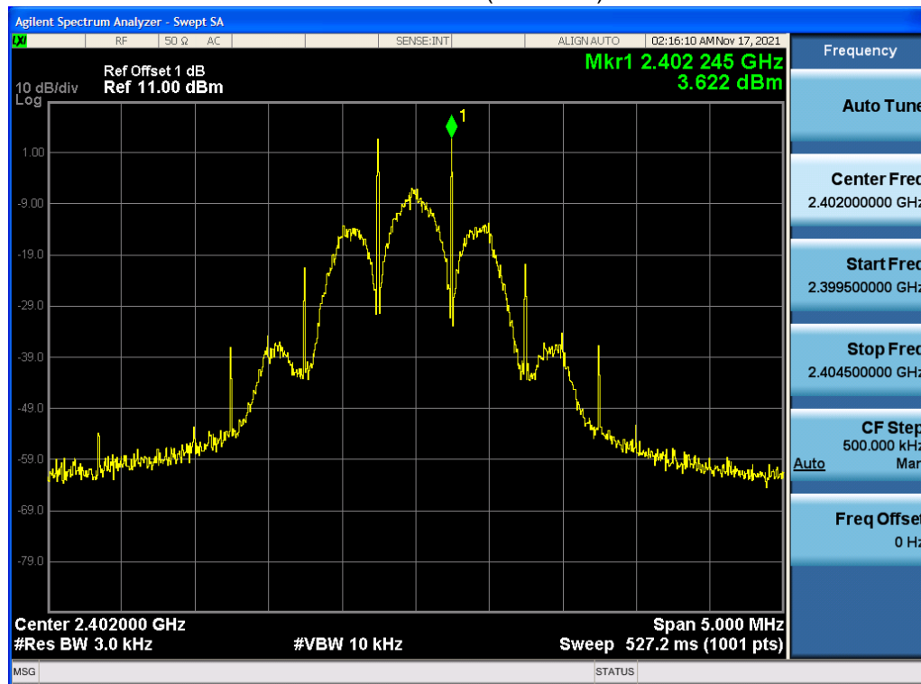
Mode 3 CH00(2402MHz)
