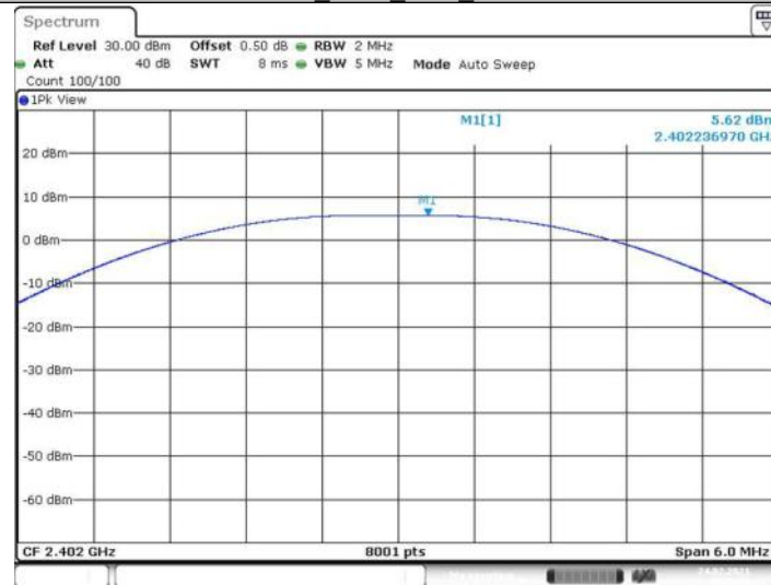
BLE_125K Ant1 2402
