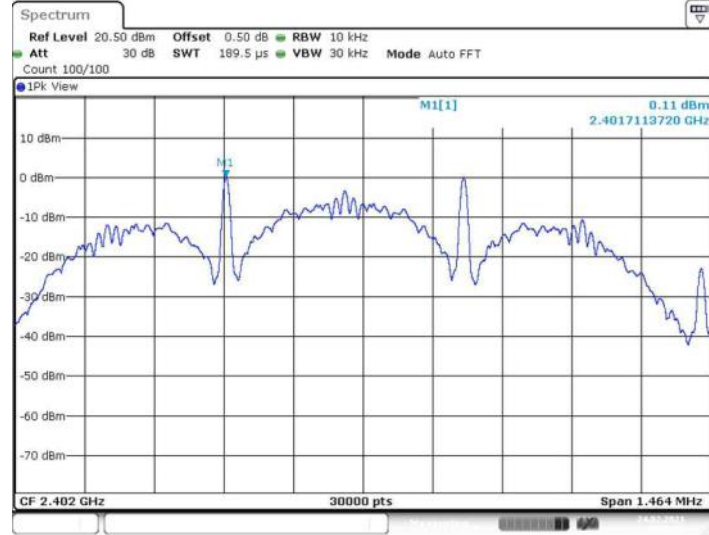
BLE_125K_Ant1_2402
