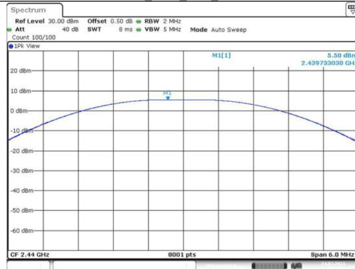
BLE_125K Ant1 2440
