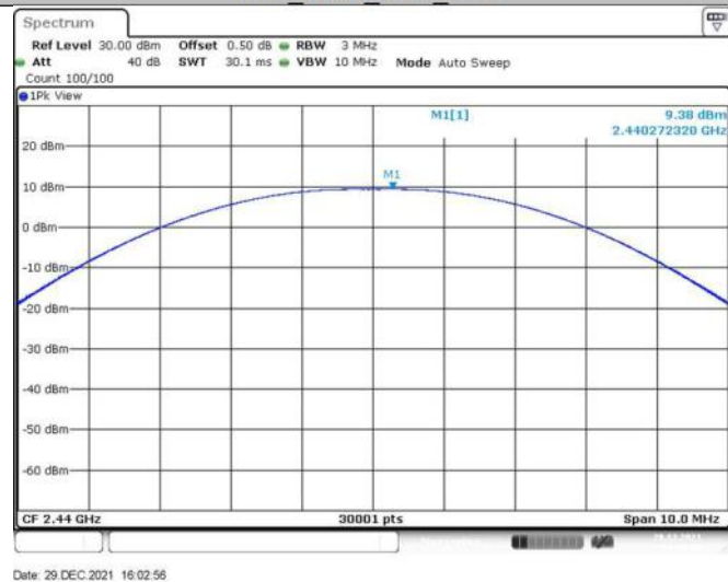
BLE_125K_Ant1_2440
