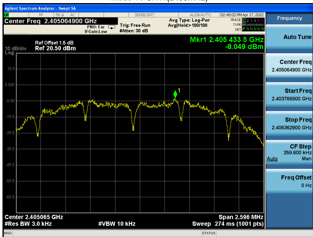
Mode 1 / CH11(2405MHz)
