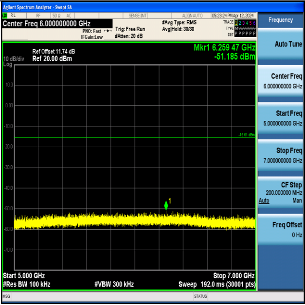
ZIGB-Ant1-2405-5000~7000-PASS
