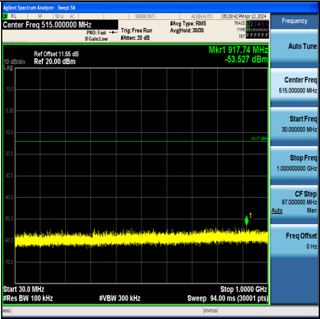
ZIGB-Ant1-2440-30~1000-PASS
