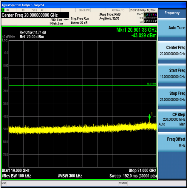
ZIGB-Ant1-2405-19000~21000-PASS
