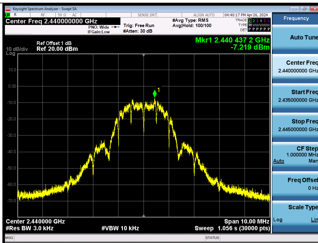
ZIGB-Ant1-2440-PASS
