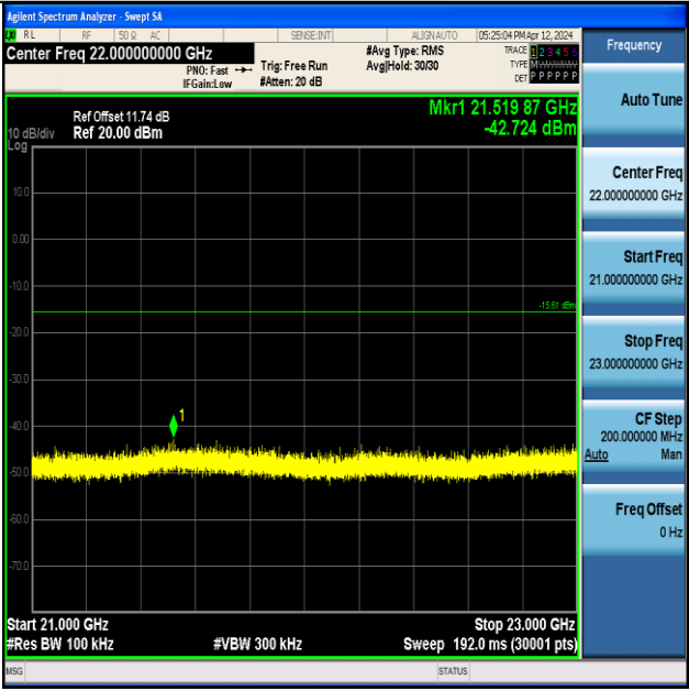
ZIGB-Ant1-2405-21000~23000-PASS
