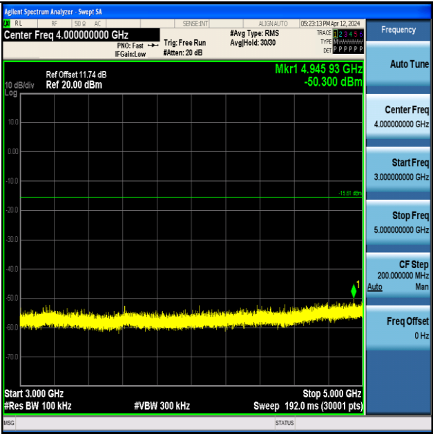
ZIGB-Ant1-2405-3000~5000-PASS
