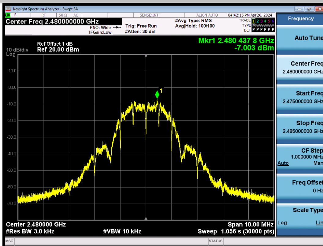
ZIGB-Ant1-2480-PASS
