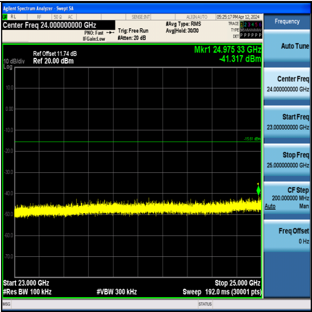
ZIGB-Ant1-2405-23000~25000-PASS
