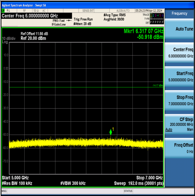
ZIGB-Ant1-2440-5000~7000-PASS
