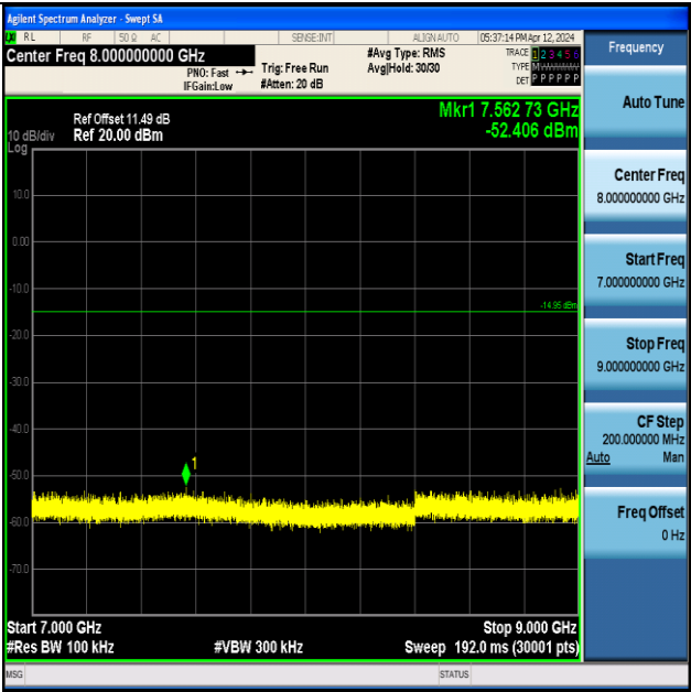
ZIGB-Ant1-2480-7000~9000-PASS
