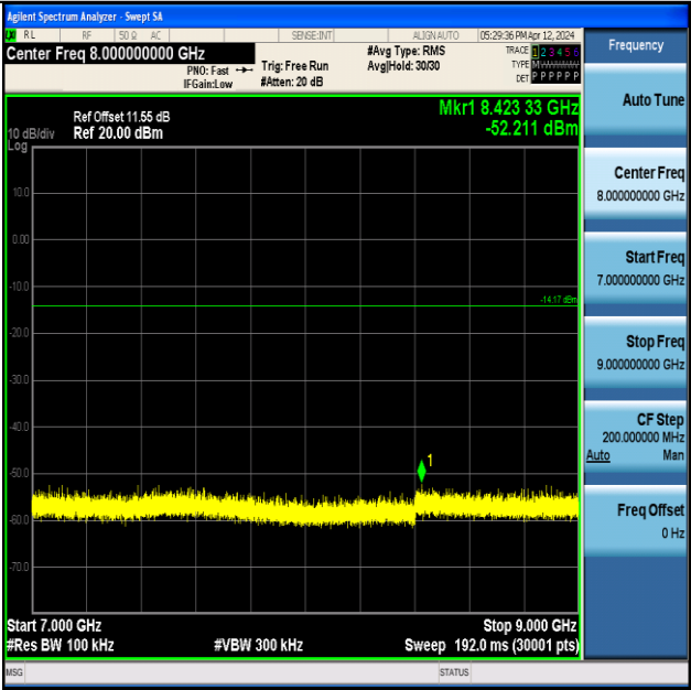
ZIGB-Ant1-2440-7000~9000-PASS
