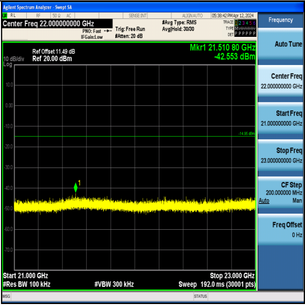
ZIGB-Ant1-2480-21000~23000-PASS
