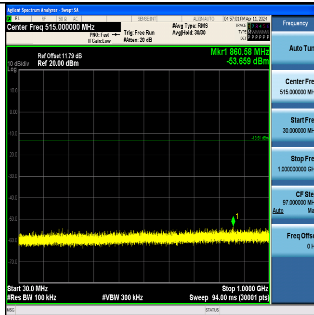
BLE_125K-Ant1-2402-30~1000-PASS
