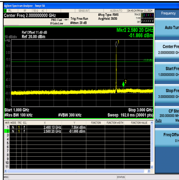
BLE_2M-Ant1-2480-1000~3000-PASS
