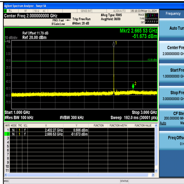
BLE_500K-Ant1-2402-1000~3000-PASS
