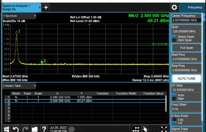
Mode 1 CH39 (2480MHz)
