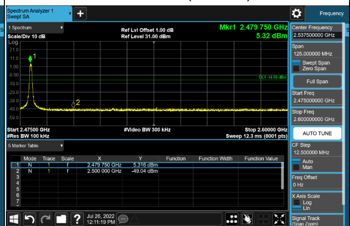
Mode 4 CH39 (2480MHz)
