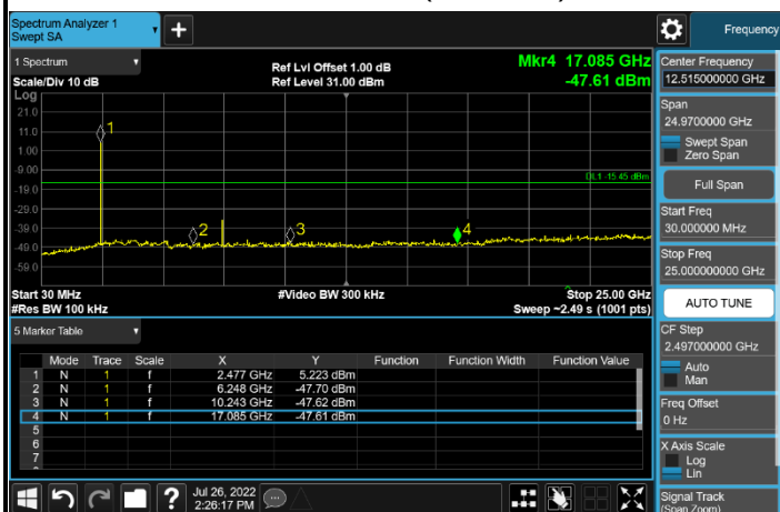
Mode 2 CH39 (2480MHz)
