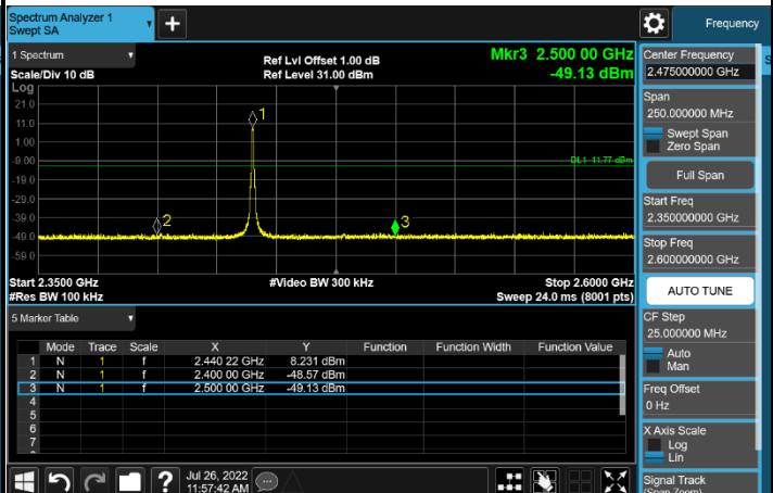
Mode 1 CH19 (2440MHz)
