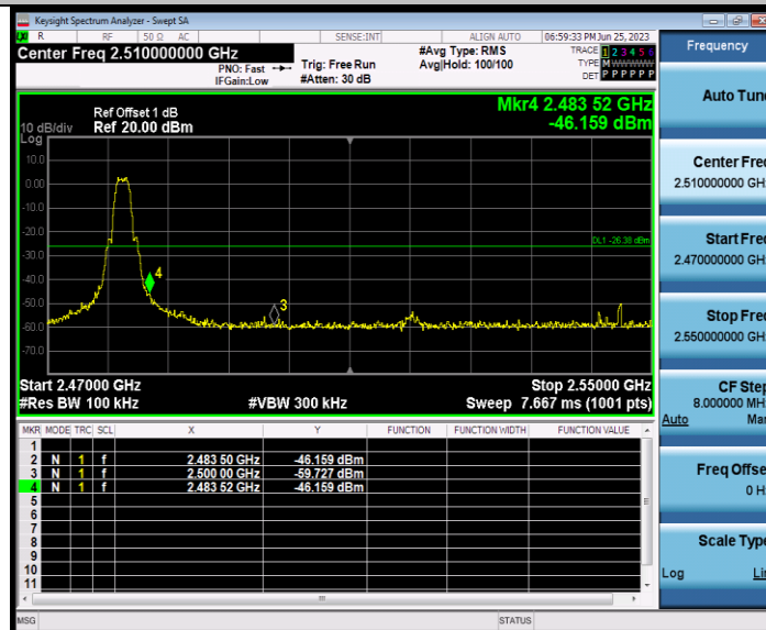
ZIGB_Ant1_High_2480
