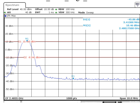
BLE_500k_High_Channel
