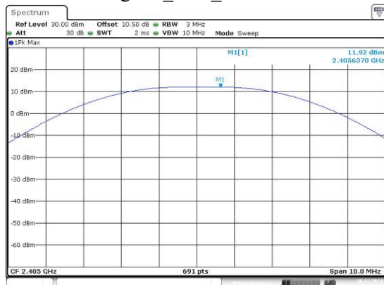
ZigBee_Low_Channel
