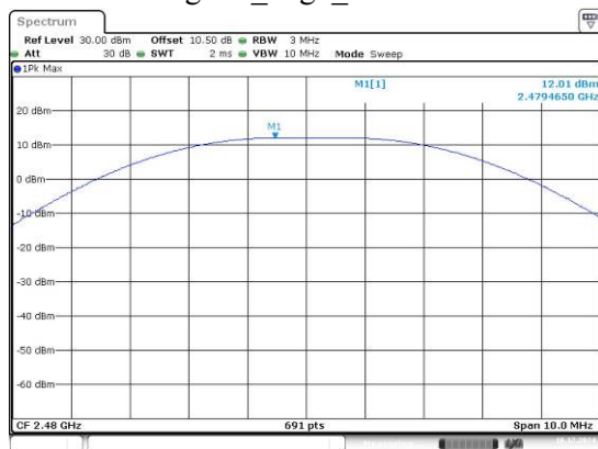
ZigBee_High_Channel
