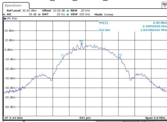
BLE_500k_Middle_Channel
