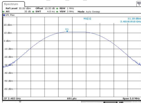
BLE_125k_Low_Channel
