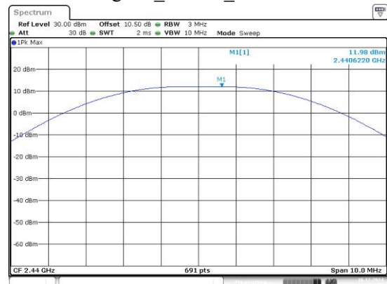
ZigBee_Middle_Channel
