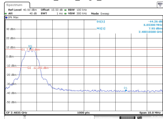
BLE_125k_High_Channel
