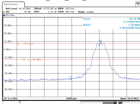
BLE_125k_Low_Channel
