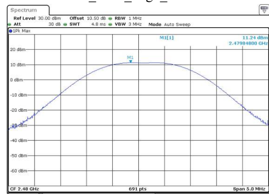
BLE_500k_High_Channel
