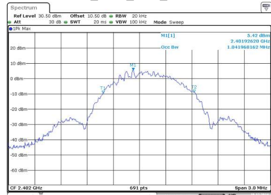
BLE_500k_Low_Channel
