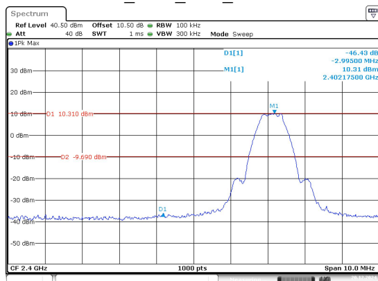
BLE_500k_Low_Channel
