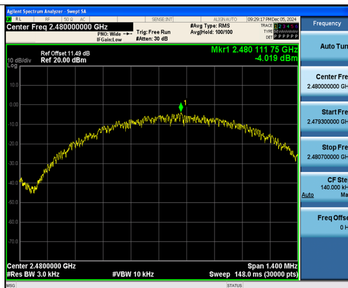
BLE_1M-Ant1-2480-PASS
