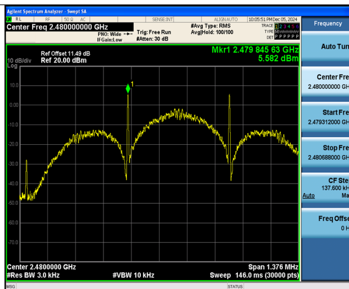
BLE_125K-Ant1-2480-PASS
