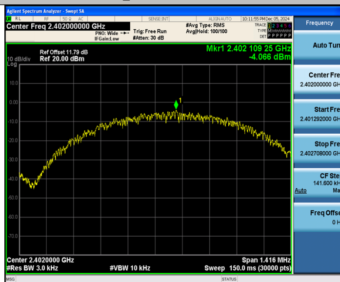
BLE_500K-Ant1-2402-PASS
