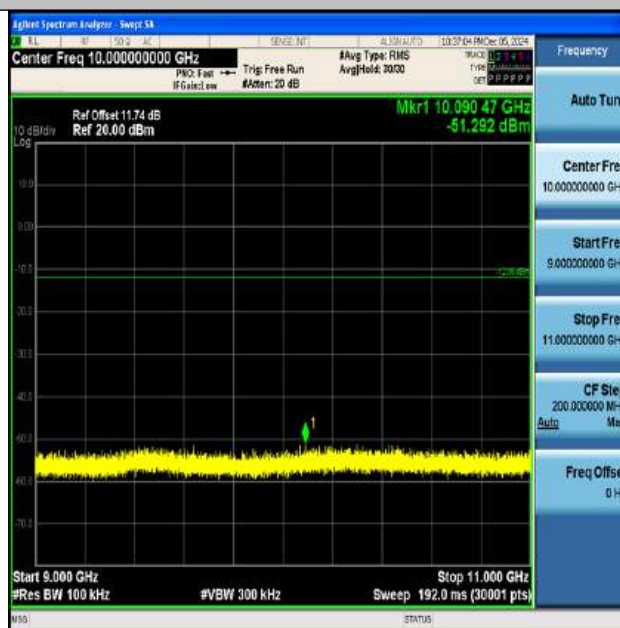
ZIGB-Ant1-2405-9000~11000-PASS
