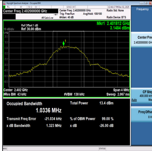
BLE_1M-Ant1-2402
