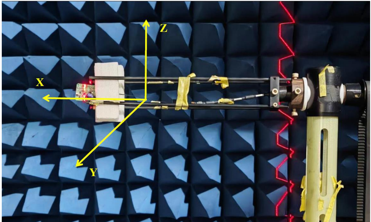
Antenna setup photo:
