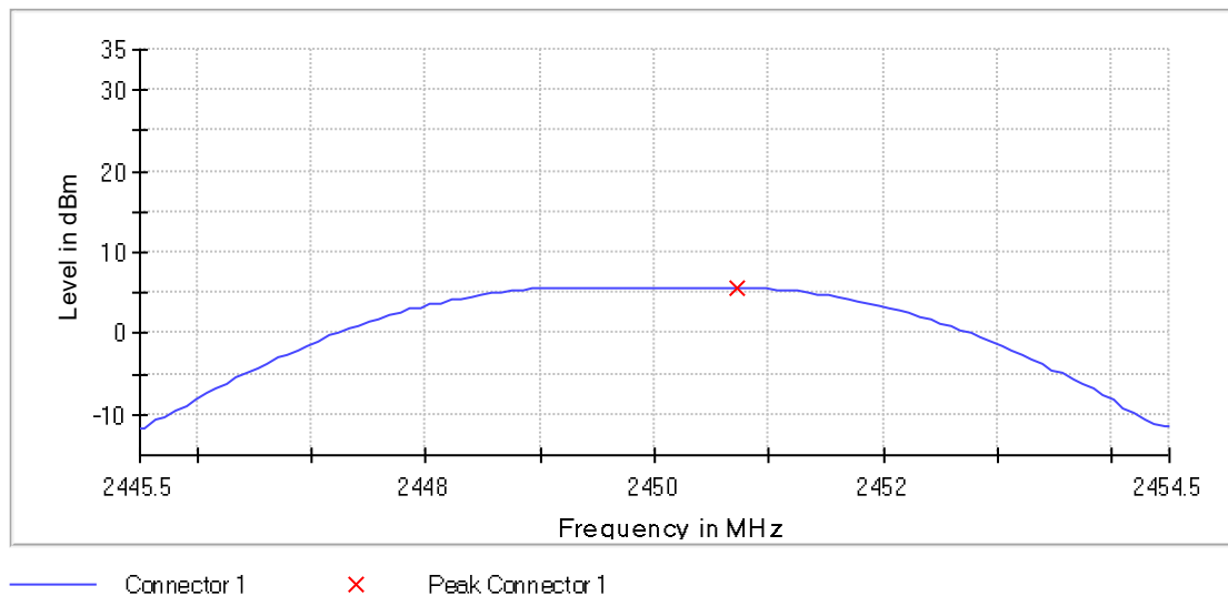
Data of 2450MHz
