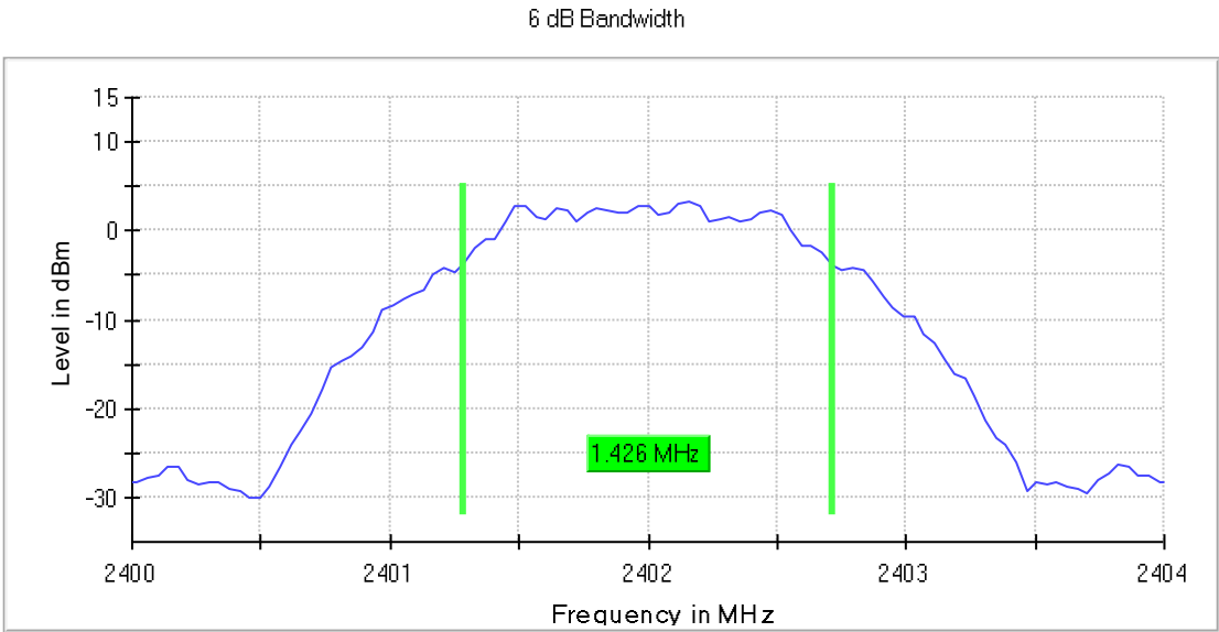
6dB Occupied Bandwidth Mode 1 / CH0 (2402MHz)
