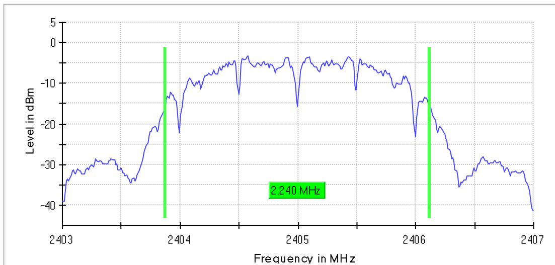
99% Occupied Bandwidth Mode 2 / CH11 (2405 MHz)
