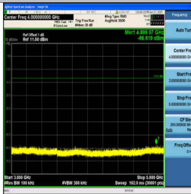
BLE_2M-Ant1-2480-3000~5000-PASS
