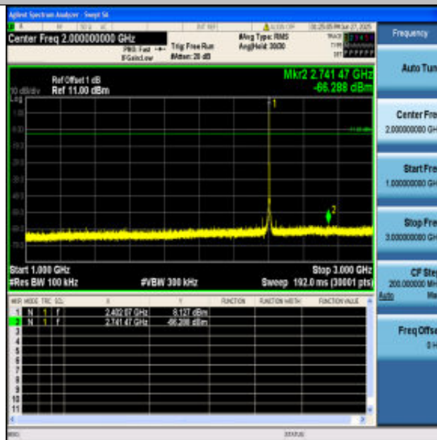
BLE_1M-Ant1-2402-1000~3000-PASS
