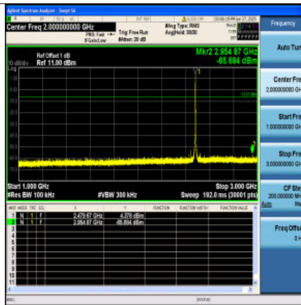
BLE_2M-Ant1-2480-1000~3000-PASS
