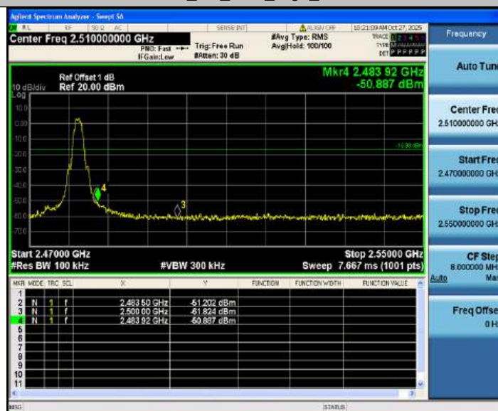
BLE_125K_Ant1_Low_2402
