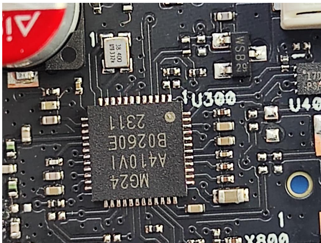
FIGURE 10 SENSOR (SC100B/02 SR TRANSCEIVER WH) CHIP & CRYSTAL
