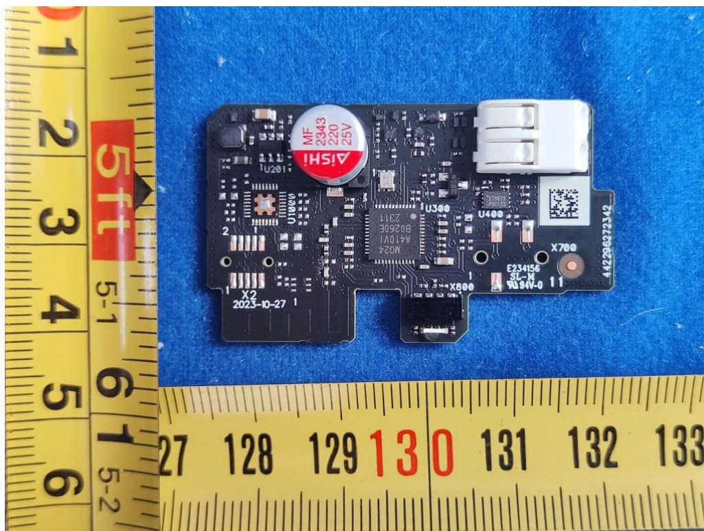
FIGURE 8 SENSOR (SC100B/02 SR TRANSCEIVER WH) MAINBOARD FRONT
