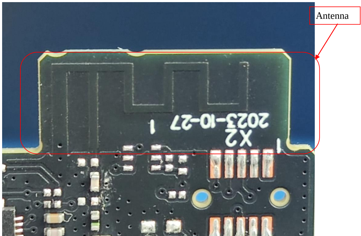
FIGURE 11 SENSOR (SC100B/02 SR TRANSCEIVER WH) ANTENNA
