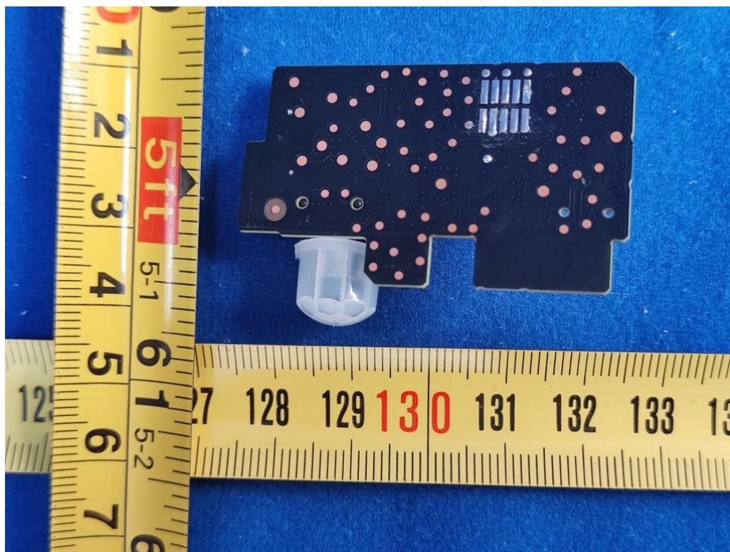
FIGURE 10 SENSOR (SC200B/02 SR SENSOR WH) CHIP & CRYSTAL
