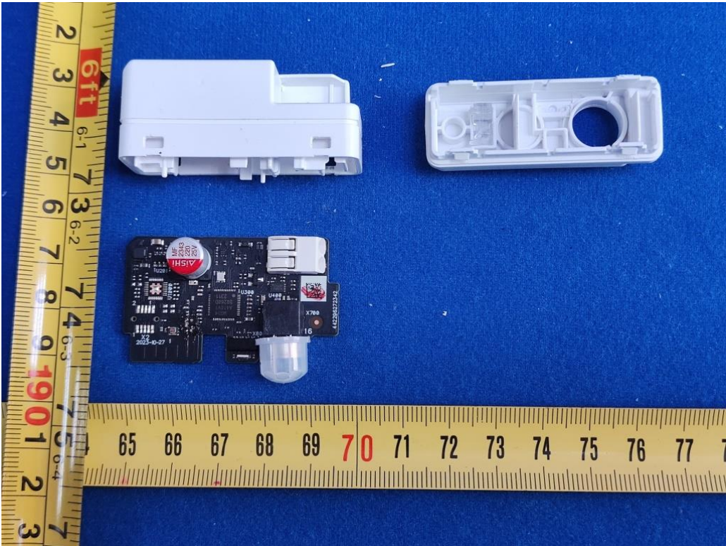
FIGURE 8 SENSOR (SC200B/02 SR SENSOR WH) MAINBOARD FRONT
