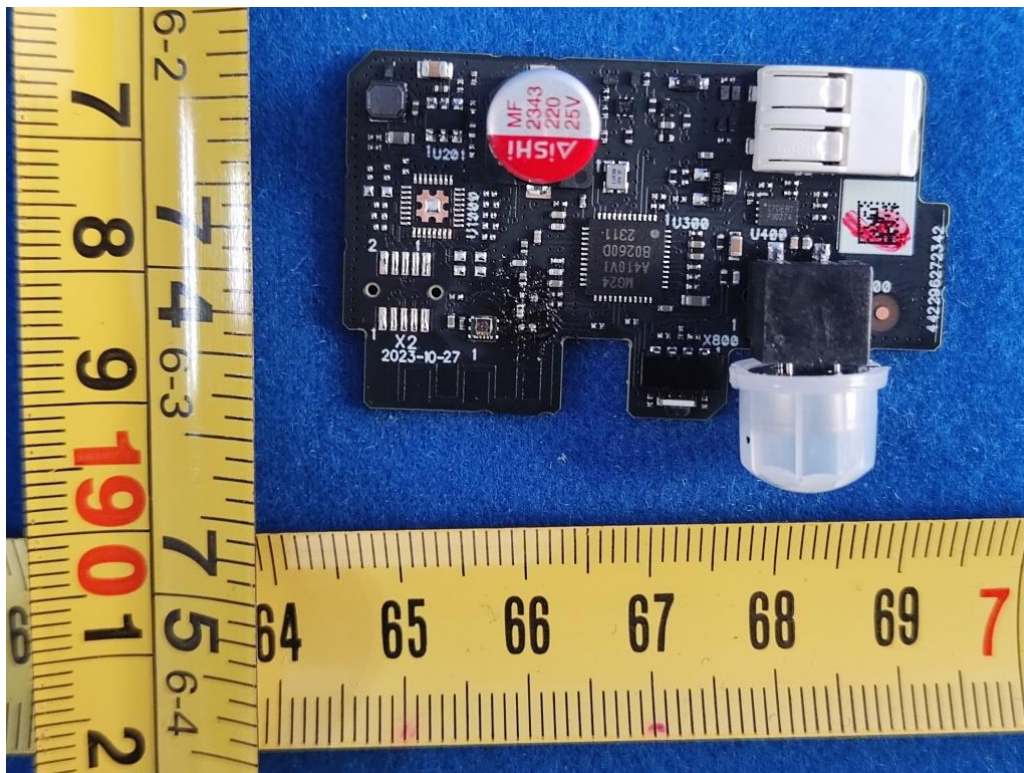
FIGURE 19 SENSOR (SC200B/02 SR SENSOR BL) MAINBOARD FRONT
