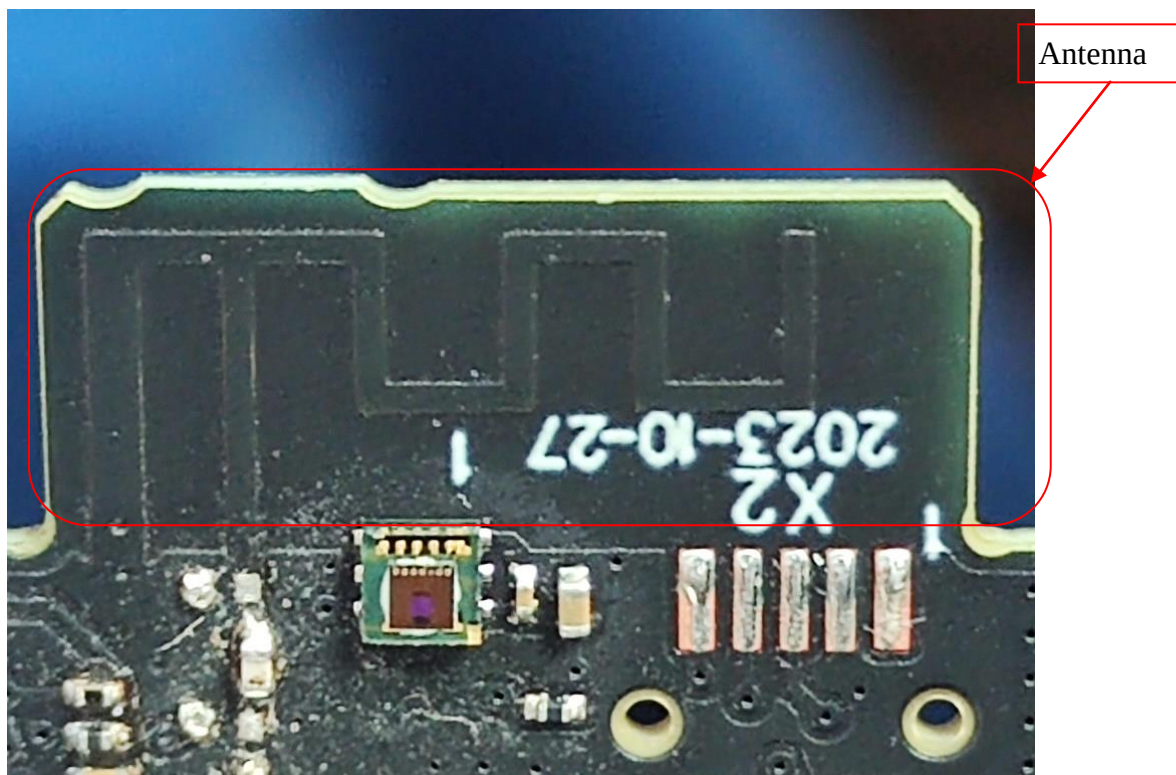
FIGURE 22 SENSOR (SC200B/02 SR SENSOR BL) ANTENNA
