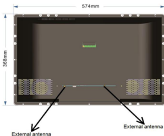
Back View of AIOT-01
