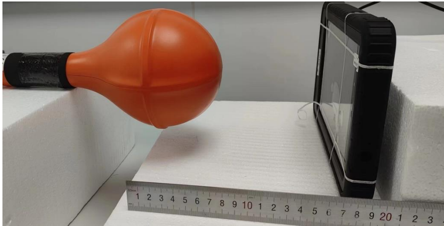
E-Field Test Setup Photo of Position E (20cm)
