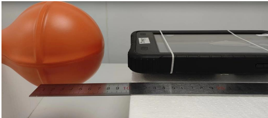
E-Field Test Setup Photo of Position B (15cm)
