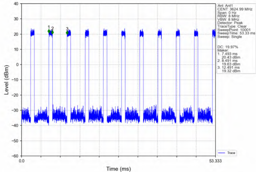
n48_30kHz_SISO_NTNV_30MHz_CP-OFDM_16_QAM_3624.99MHz_Inner_Full_Ant1
