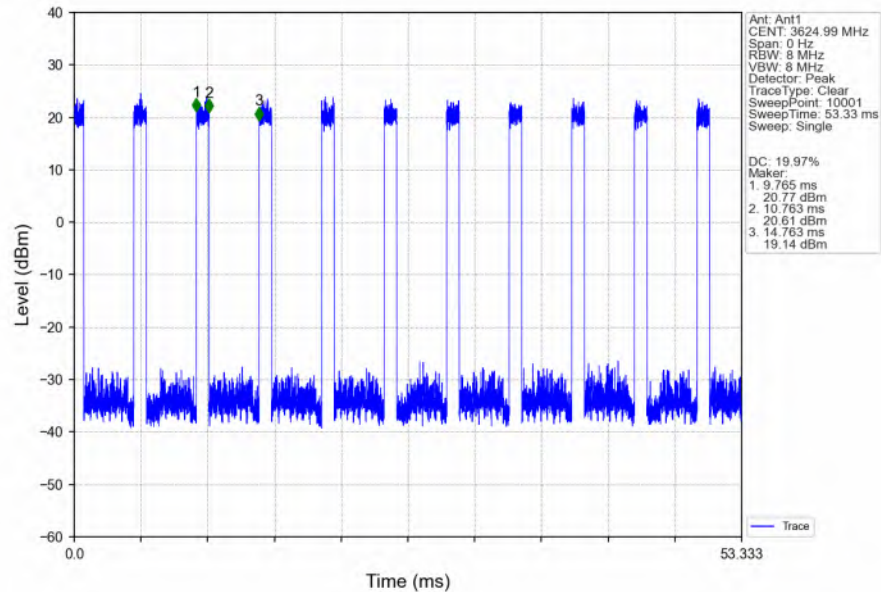
n48_30kHz_SISO_NTNV_30MHz_CP-OFDM QPSK_3624.99MHz_Inner_Full_Ant1
