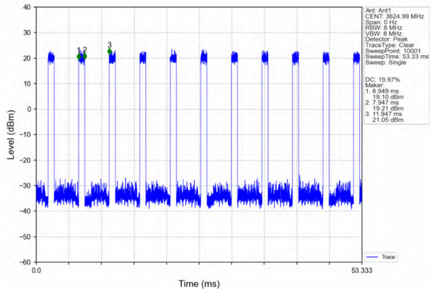
n48_30kHz_SISO_NTNV_30MHz_CP-OFDM 64 QAM_3624.99MHz_Inner_Full_Ant1
