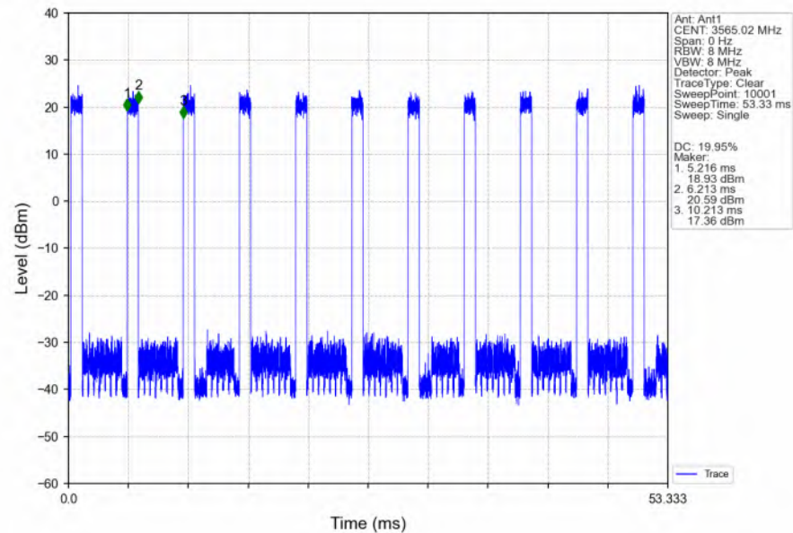
n48_30kHz_SISO_NTNV_30MHz_CP-OFDM_16_QAM_3565.02MHz_Inner_Full_Ant1
