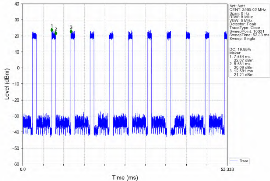
n48_30kHz_SISO_NTNV_30MHz_CP-OFDM 64 QAM_3565.02MHz_Inner_Full_Ant1
