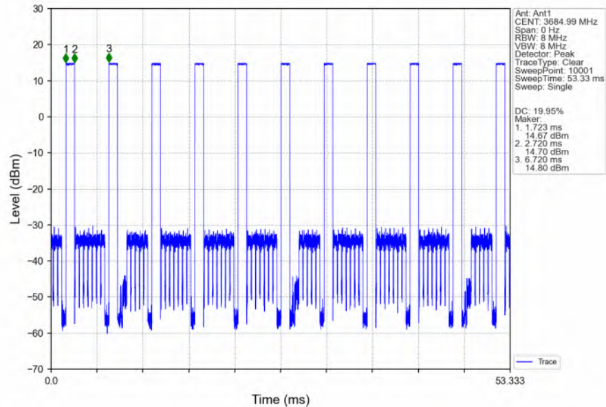
n48_30kHz_SISO_NTNV_30MHz_CP-OFDM_16_QAM_3684.99MHz_Inner_Full_Ant1
