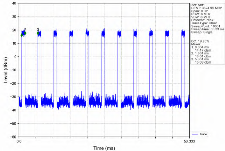
n48_30kHz_SISO_NTNV_30MHz_CP-OFDM 256 QAM_3624.99MHz_Inner_Full_Ant1
