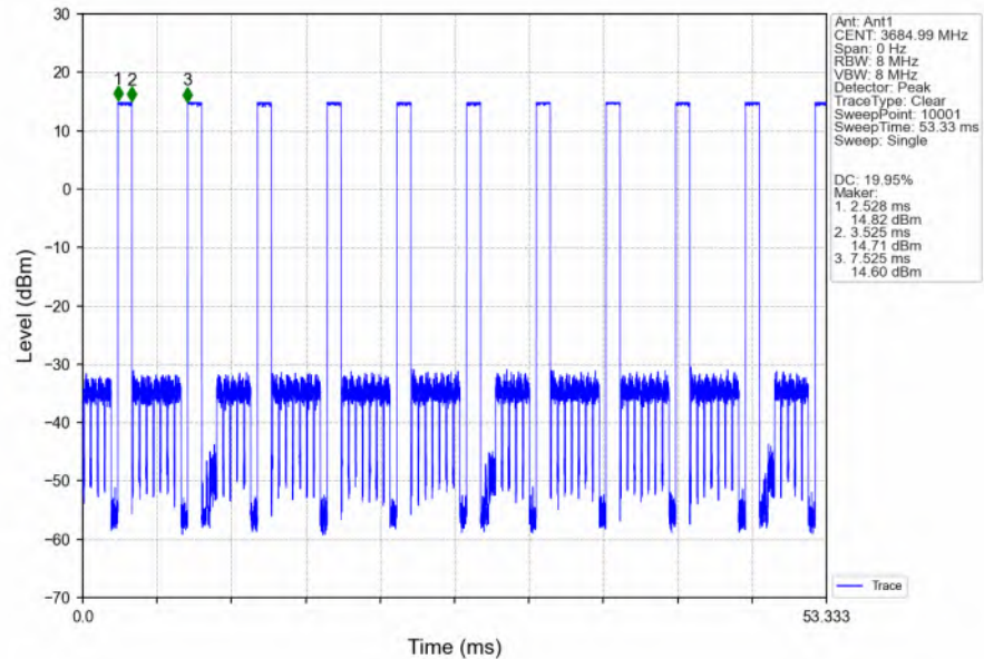
n48_30kHz_SISO_NTNV_30MHz_CP-OFDM_64_QAM_3684.99MHz_Inner_Full_Ant1
