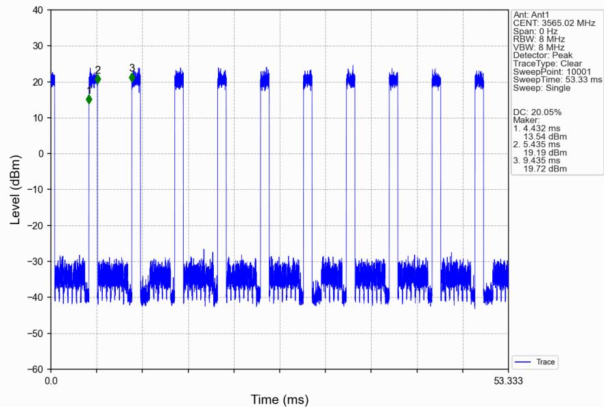
n48_30kHz_SISO_NTNV_30MHz_CP-OFDM QPSK_3565.02MHz_Inner_Full_Ant1
