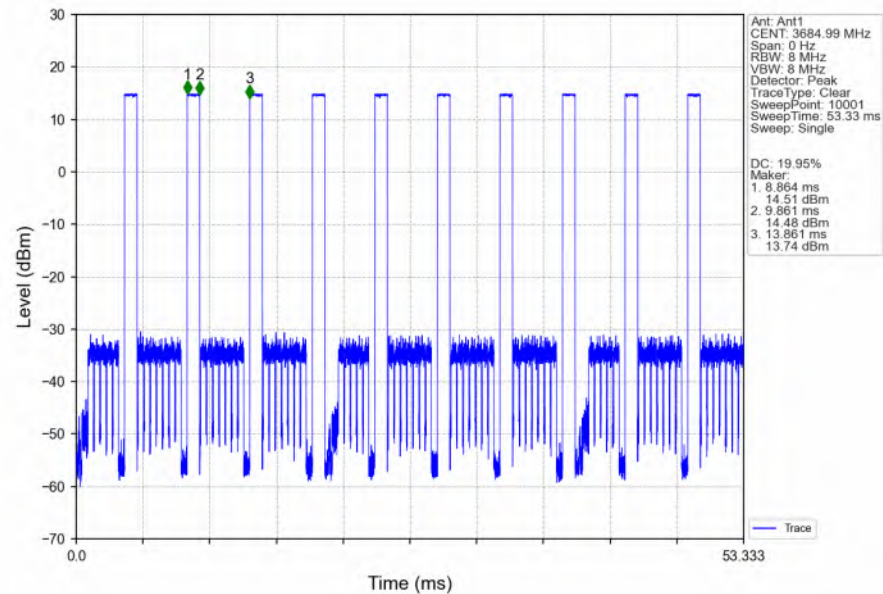
n48_30kHz_SISO_NTNV_30MHz_CP-OFDM QPSK_3684.99MHz_Inner_Full_Ant1
