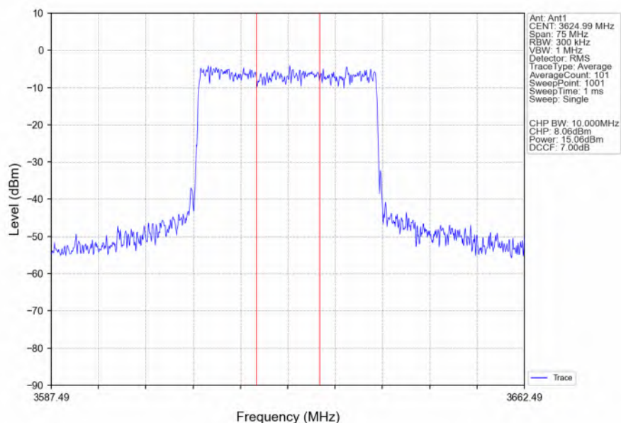
n48_30kHz_SISO_NTNV_30MHz_CP-OFDM 64 QAM_3624.99MHz_Inner_Full_Ant1
