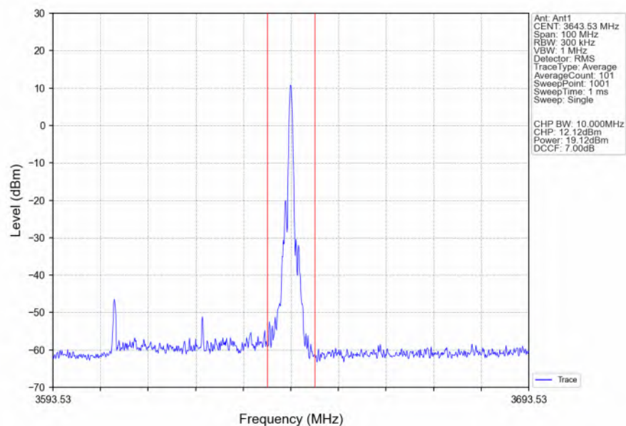
n48_30kHz_SISO_NTNV_40MHz_DFT-s-OFDM 256 QAM_3624.99MHz_Inner_1RB_Right_Ant1
