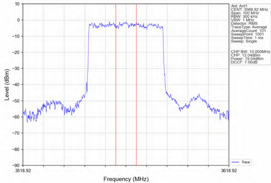
n48_30kHz_SISO_NTNV_40MHz_DFT-s-OFDM PI/2 BPSK_3570MHz_Inner_Full_Ant1
