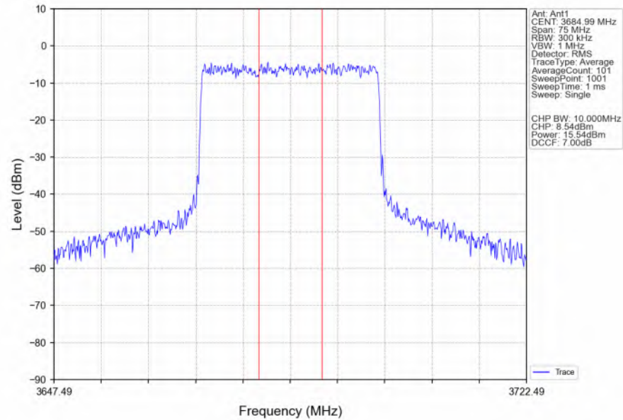
n48_30kHz_SISO_NTNV_30MHz_CP-OFDM QPSK_3684.99MHz_Inner_Full_Ant1
