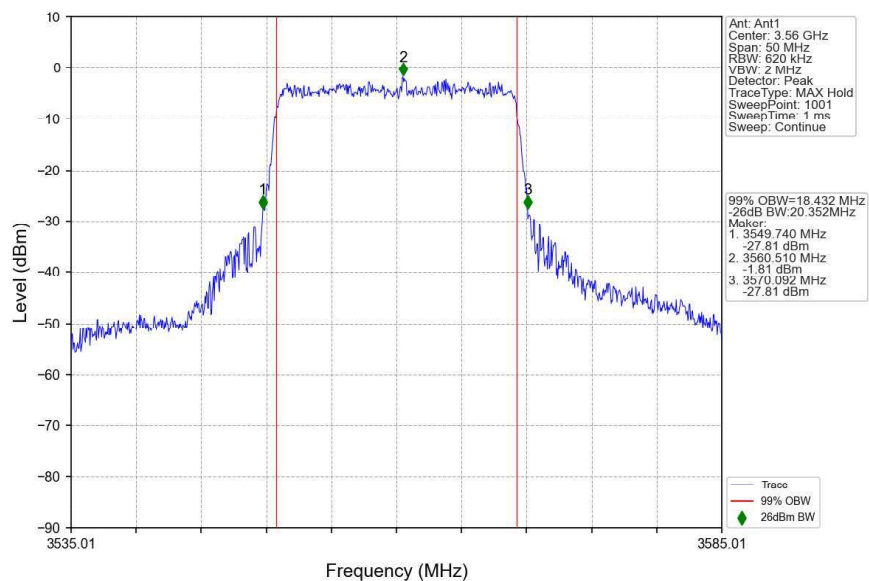
n48_30kHz_SISO_NTNV_20MHz_CP-OFDM 16 QAM_3560.01MHz_Outer_Full
