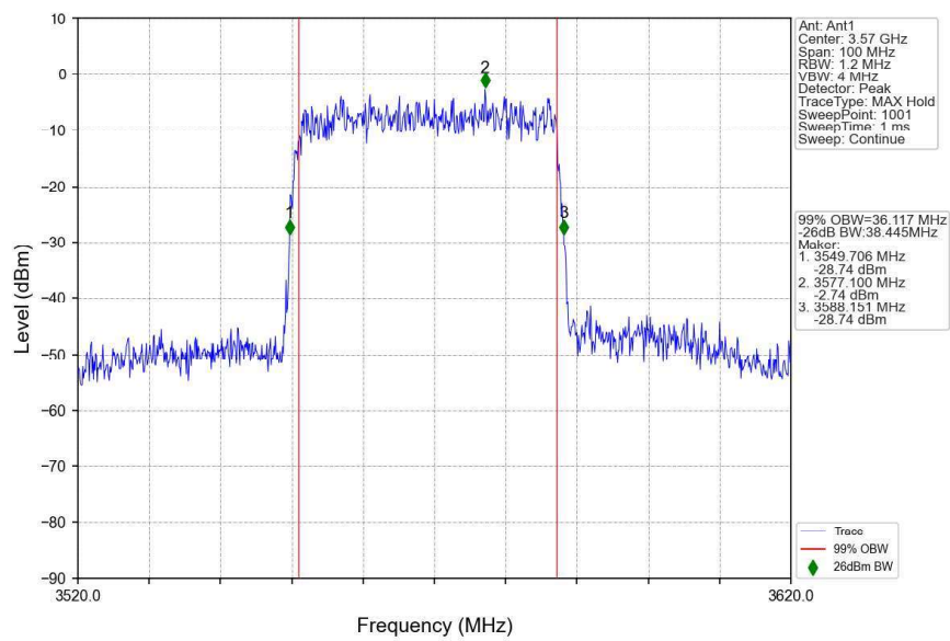
n48_30kHz_SISO_NTNV_40MHz_DFT-s-OFDM 16 QAM_3570MHz_Outer_Full
