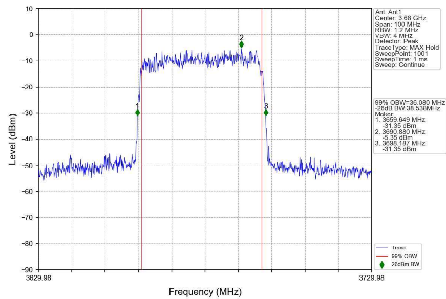
n48_30kHz_SISO_NTNV_40MHz_DFT-s-OFDM 256 QAM_3679.98MHz_Outer_Full
