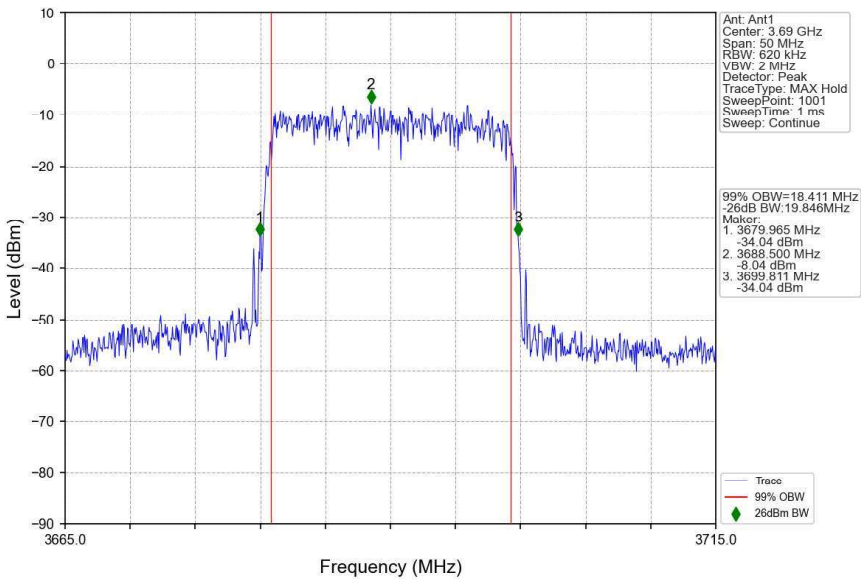
n48_30kHz_SISO_NTNV_20MHz_CP-OFDM 256 QAM_3690MHz_Outer_Full
