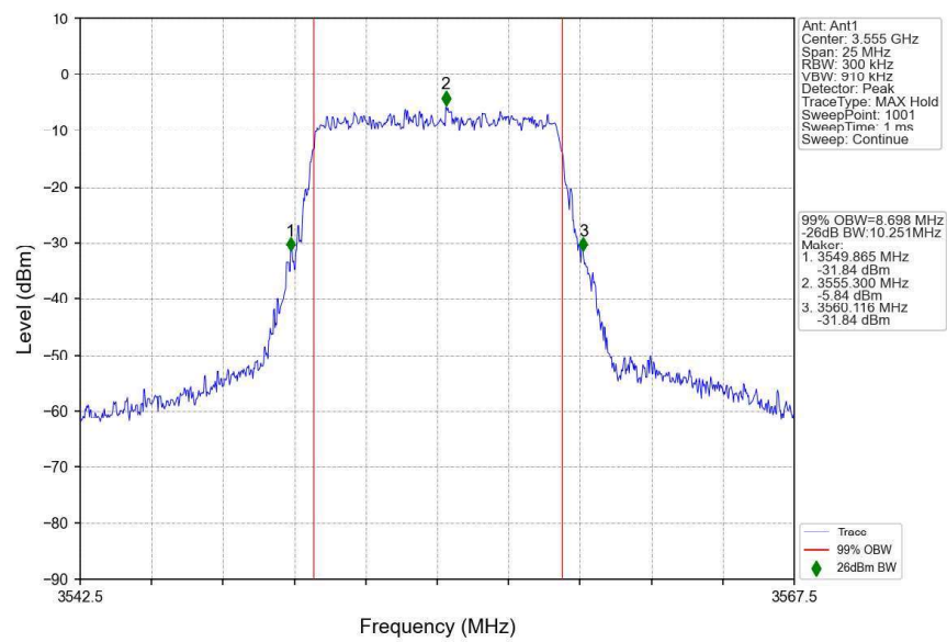
n48_30kHz_SISO_NTNV_10MHz_CP-OFDM 256 QAM_3555MHz_Outer_Full
