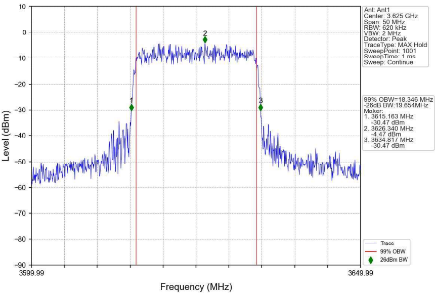
n48_30kHz_SISO_NTNV_20MHz_CP-OFDM QPSK_3624.99MHz_Outer_Full
