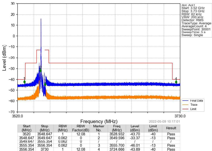
Band48_5MHz_QPSK_LCH_3552.5MHz_RB_1_0_NTNV
