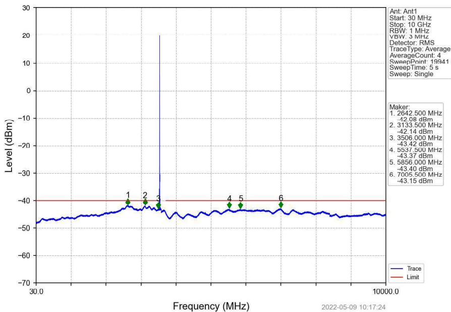
Band48_5MHz_QPSK_LCH_3552.5MHz_RB_1_0_NTNV
