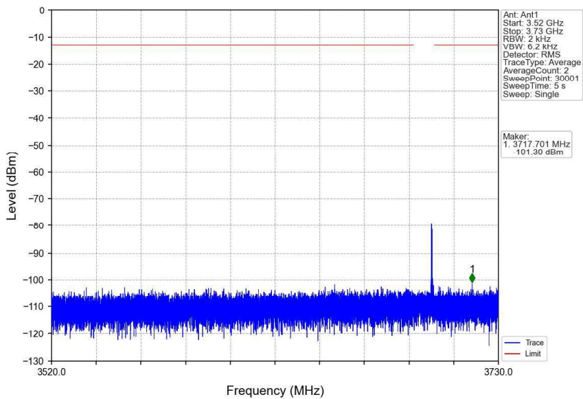
n48_30kHz_SISO_NTNV_10MHz_CP-OFDM QPSK_3694.98MHz_Inner_1RB_Right
