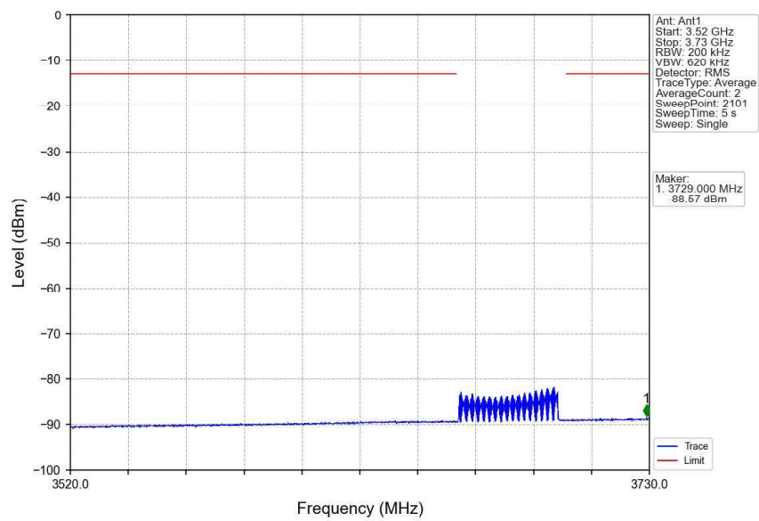
n48_30kHz_SISO_NTNV_40MHz_DFT-s-OFDM QPSK_3679.98MHz_Inner_1RB_Right
