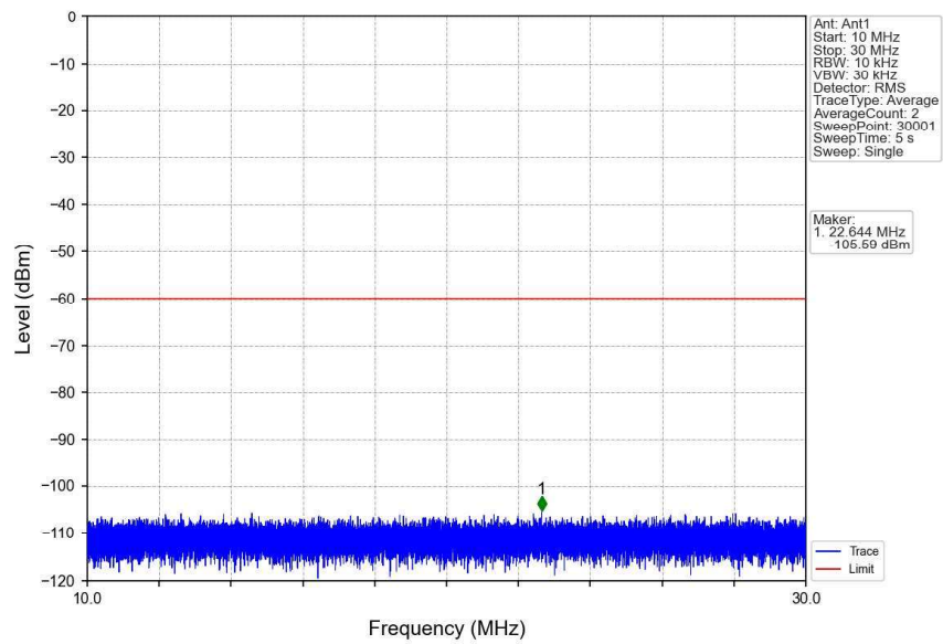
n48_30kHz_SISO_NTNV_40MHz_DFT-s-OFDM QPSK_3570MHz_Edge_1RB_Left
