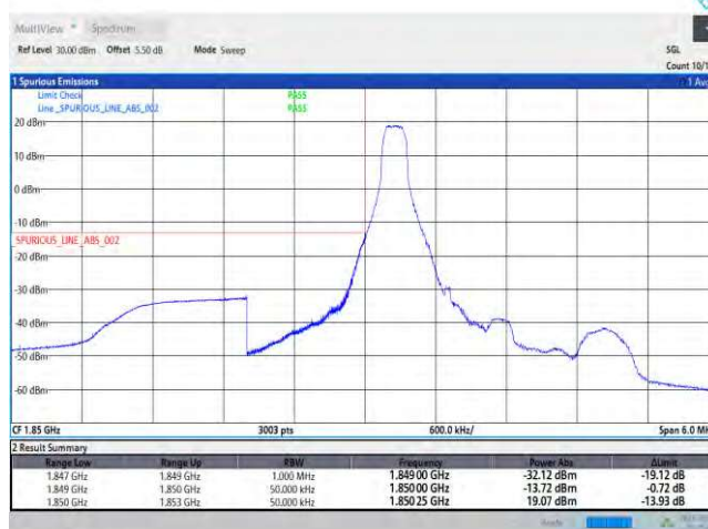
Band2-1.4MHz-QPSK-18607-6RB#0
