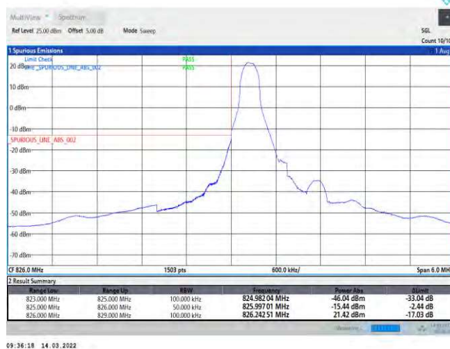
Band5-1.4MHz-QPSK-20427-6RB#0
